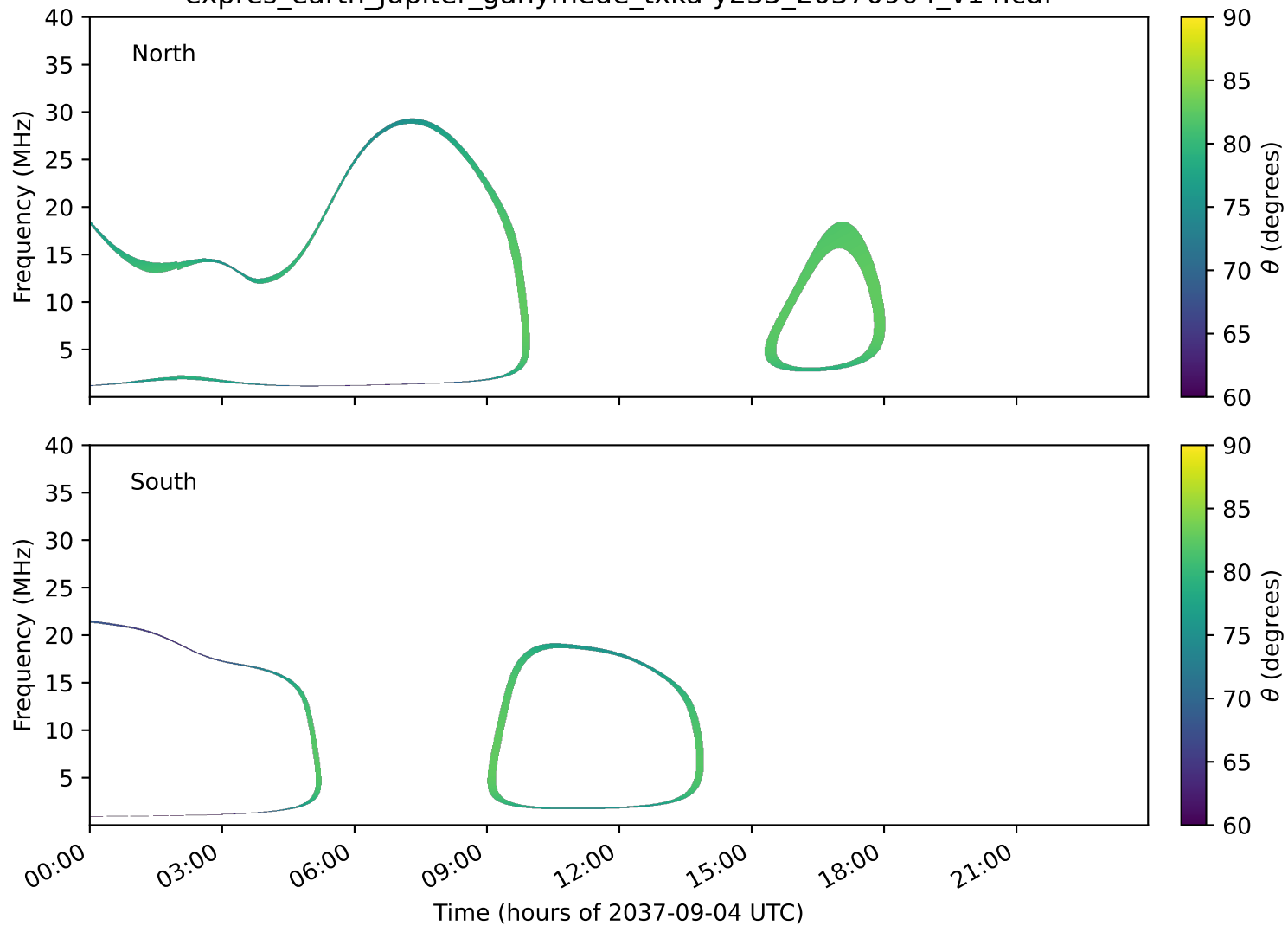
expres_earth_jupiter_ganymede_txka-y235_20370904_v14.cdf
