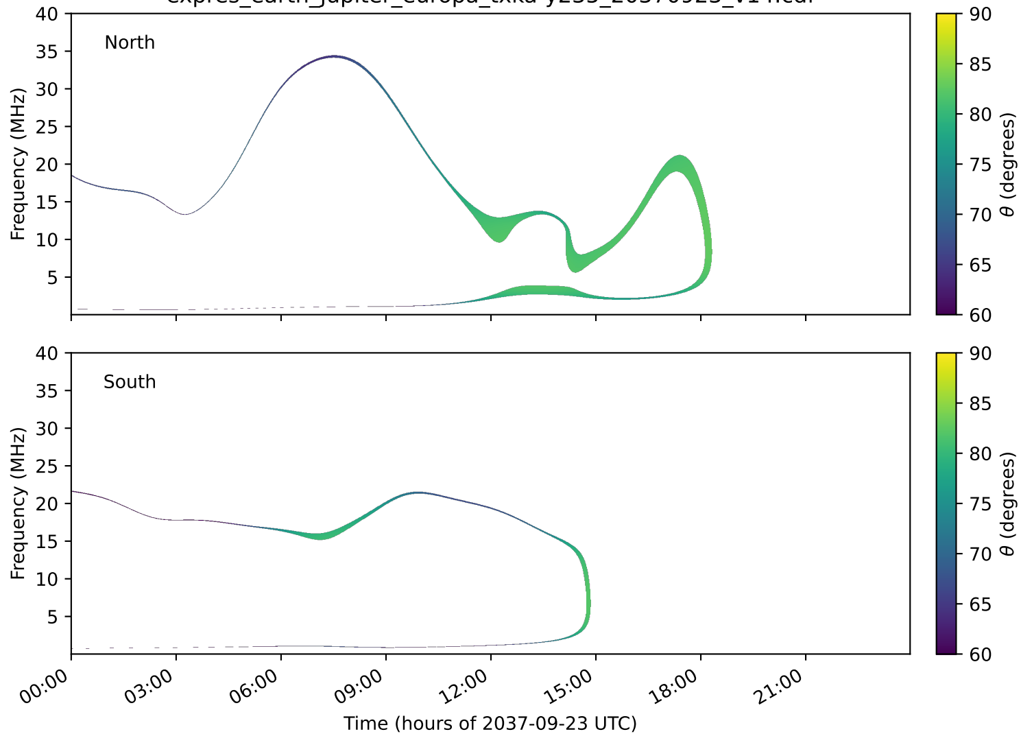
expres_earth_jupiter_europa_txka-y235_20370923_v14.cdf
