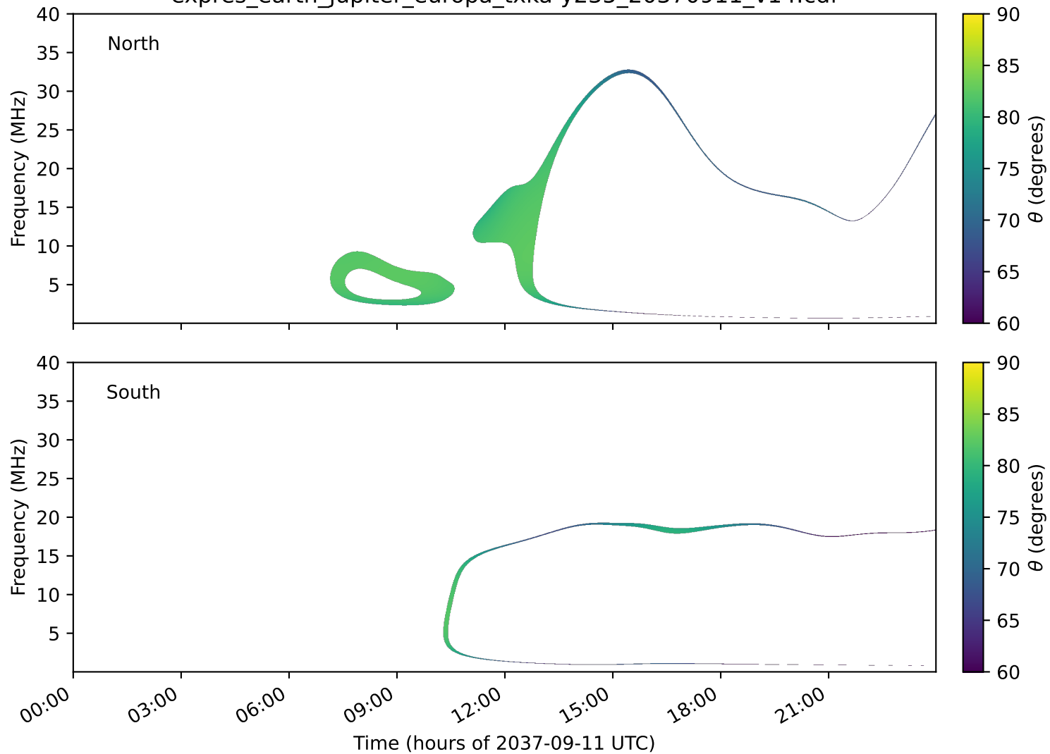
expres_earth_jupiter_europa_txka-y235_20370911_v14.cdf
