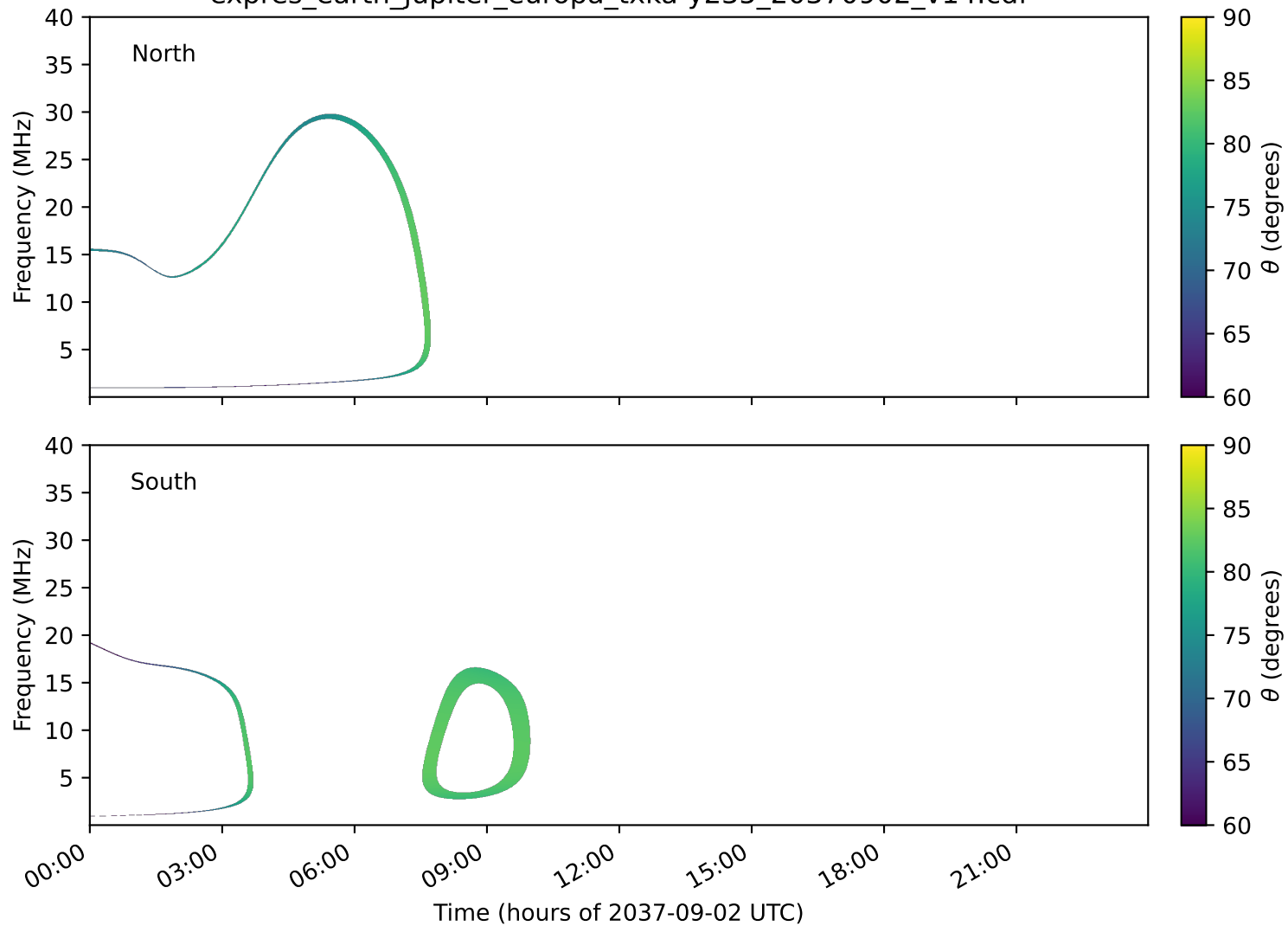
expres_earth_jupiter_europa_txka-y235_20370902_v14.cdf
