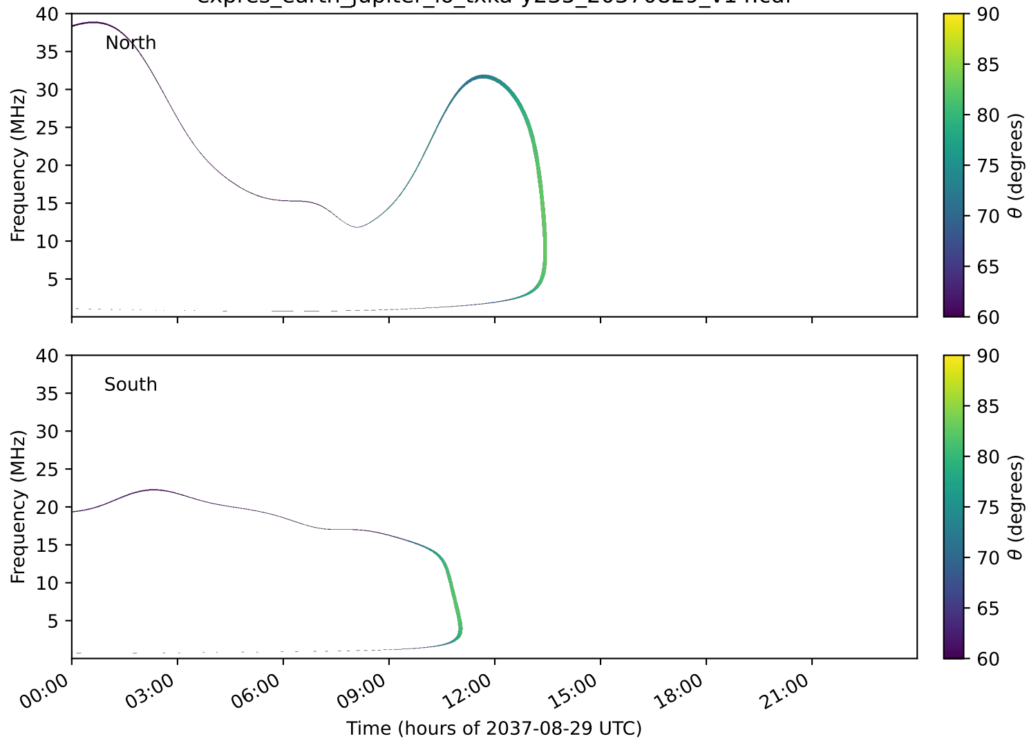
expres_earth_jupiter_io_txka-y235_20370829_v14.cdf
