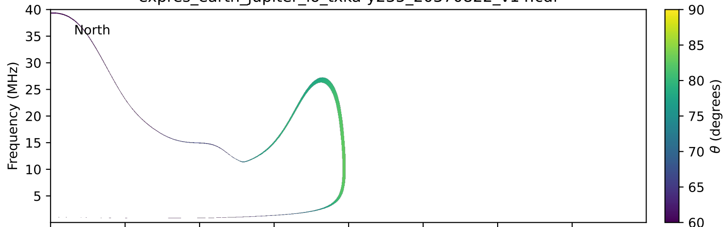
expres_earth_jupiter_io_txka-y235_20370822_v14.cdf
