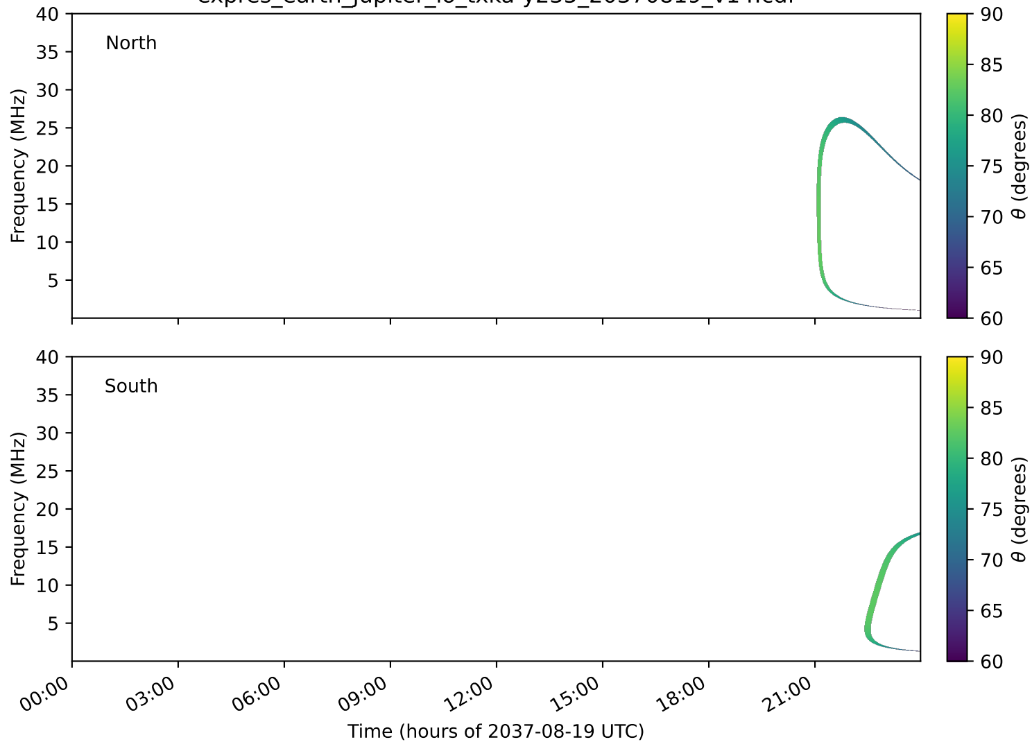
expres_earth_jupiter_io_txka-y235_20370819_v14.cdf
