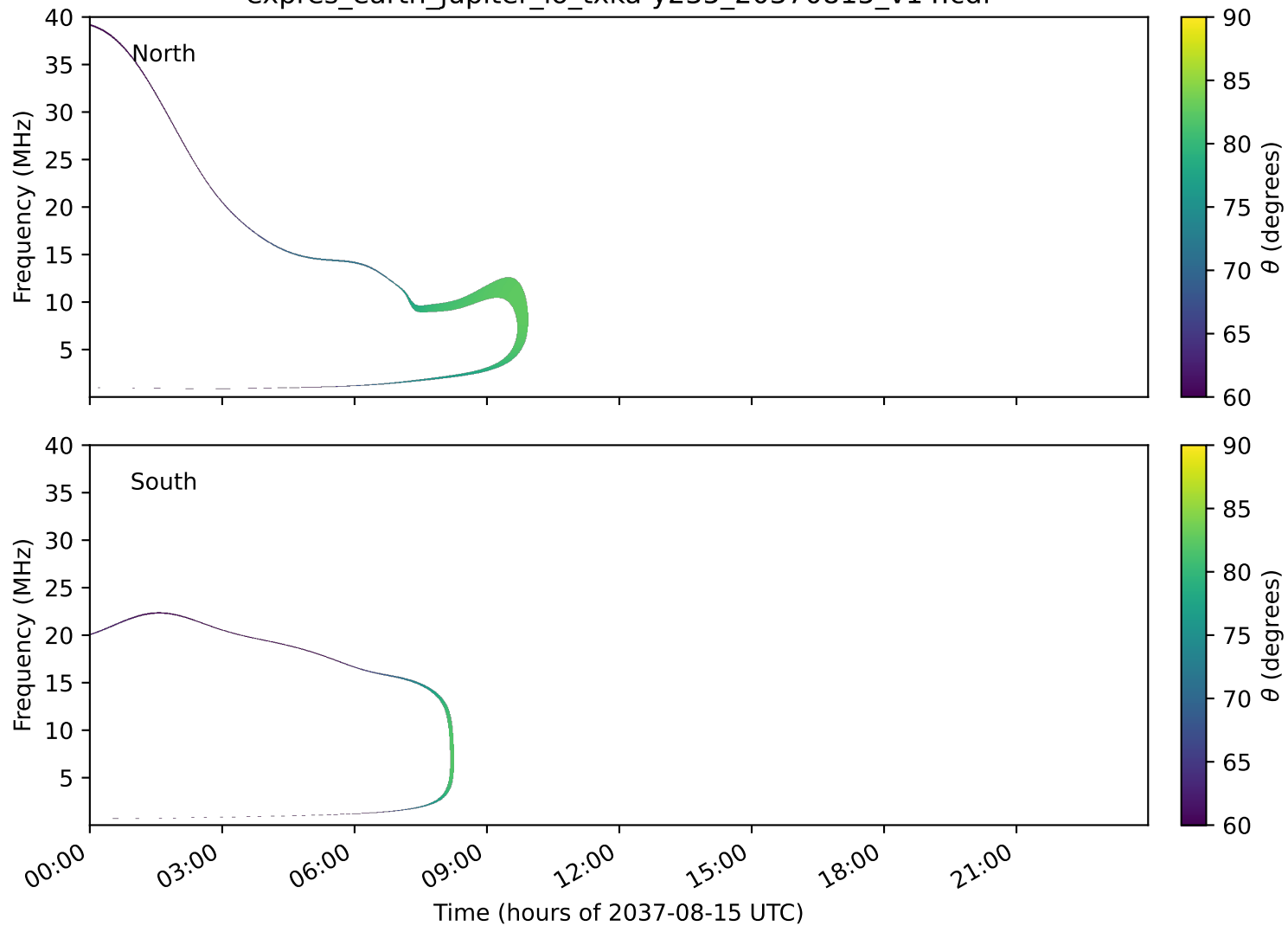
expres_earth_jupiter_io_txka-y235_20370815_v14.cdf
