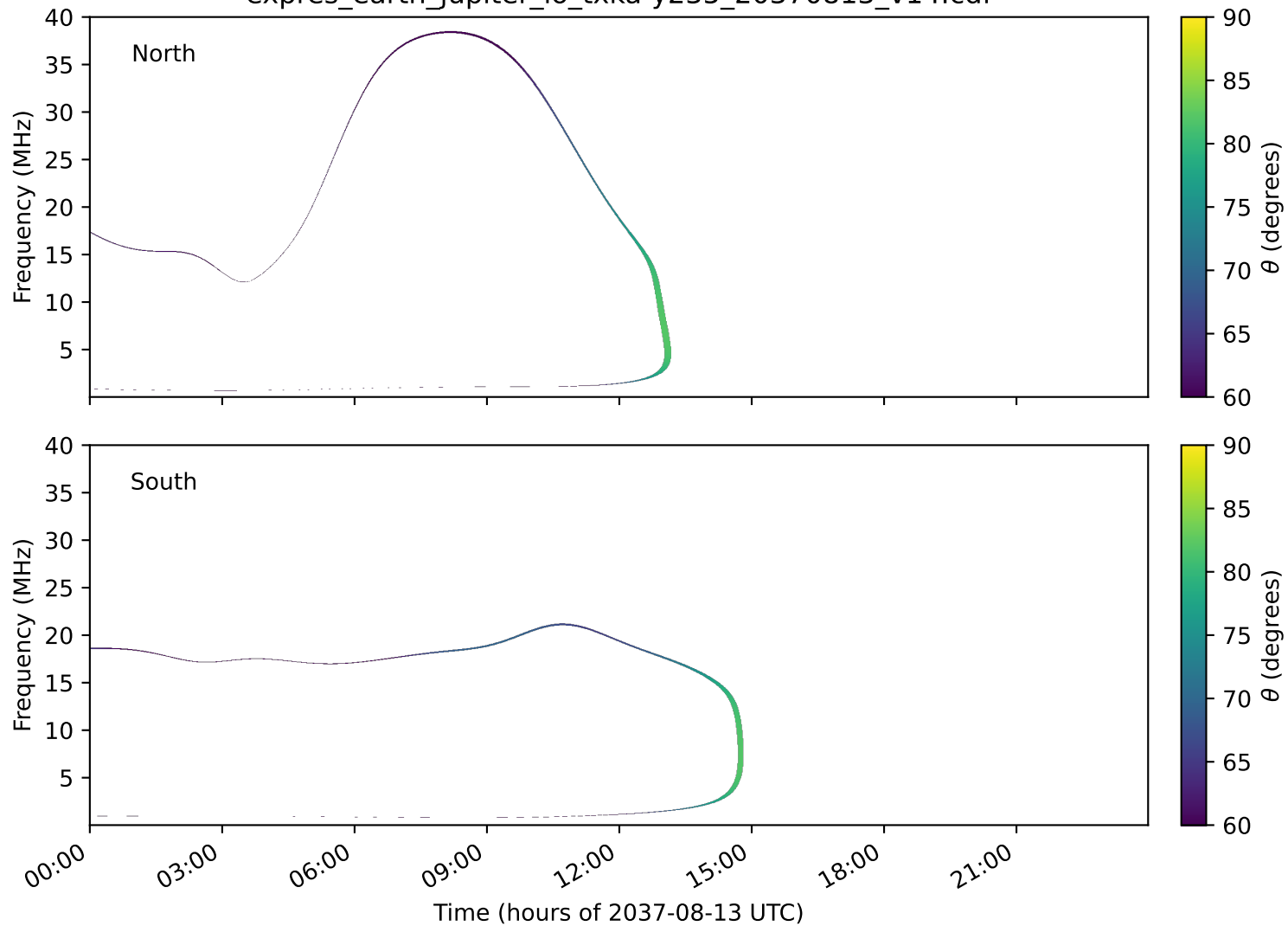
expres_earth_jupiter_io_txka-y235_20370813_v14.cdf
