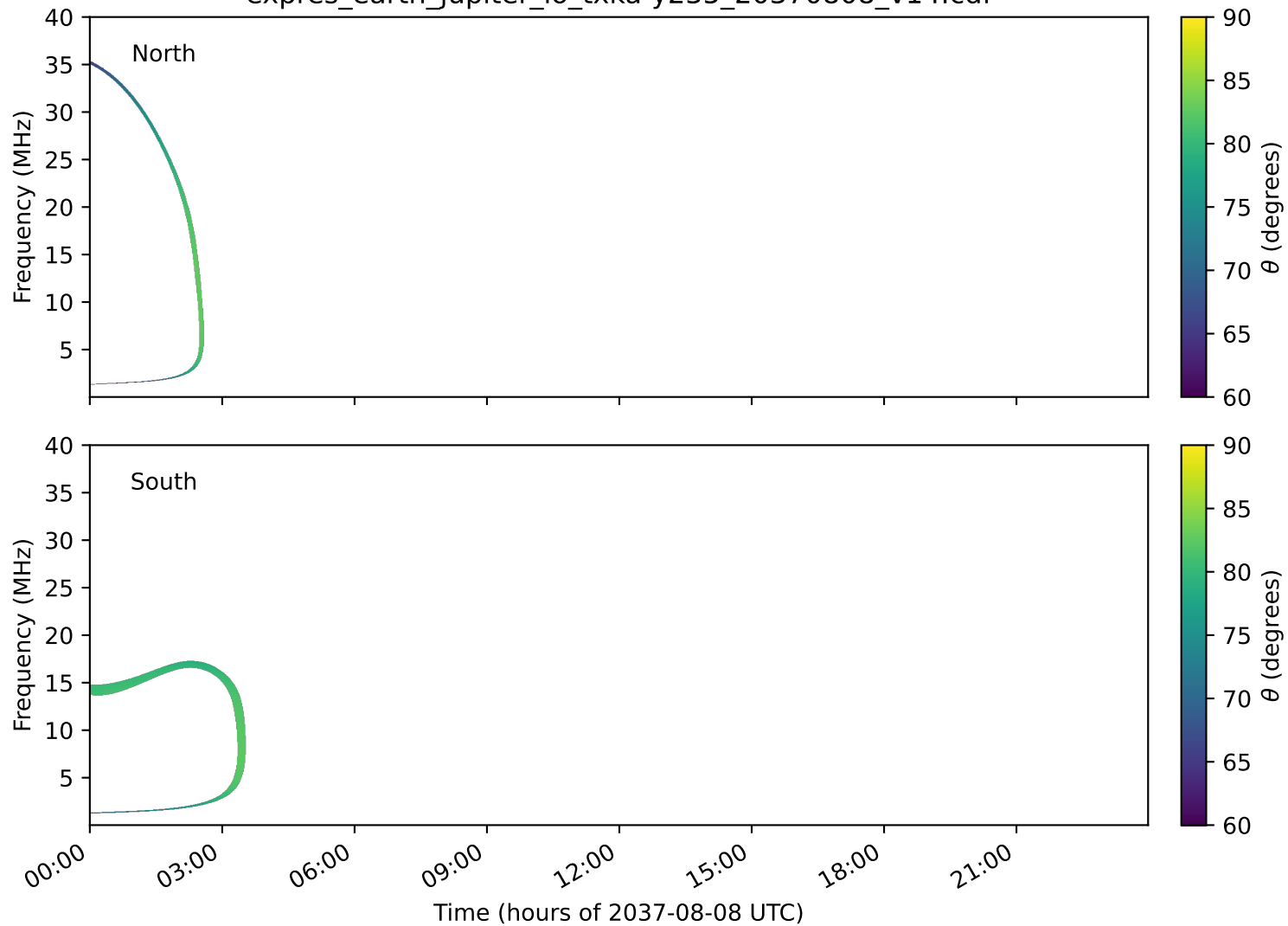
expres_earth_jupiter_io_txka-y235_20370808_v14.cdf
