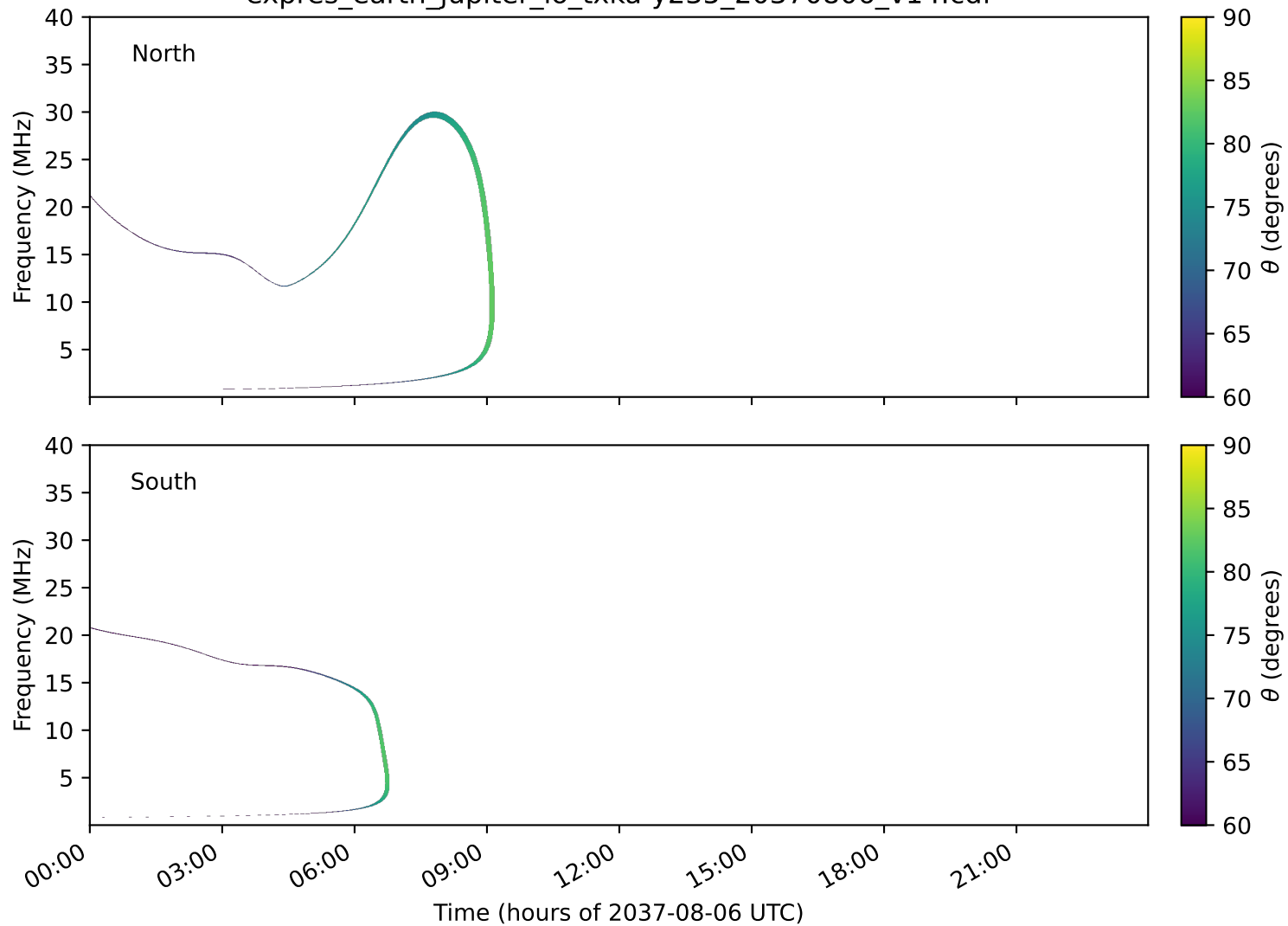
expres_earth_jupiter_io_txka-y235_20370806_v14.cdf
