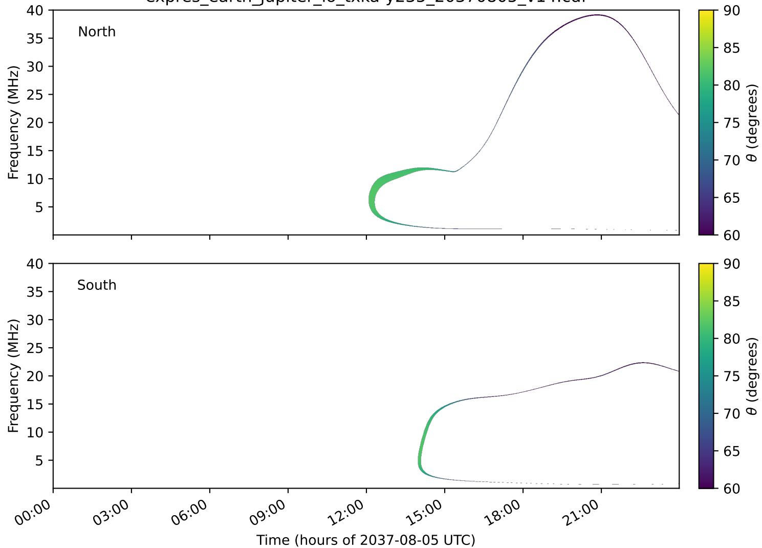
expres_earth_jupiter_io_txka-y235_20370805_v14.cdf
