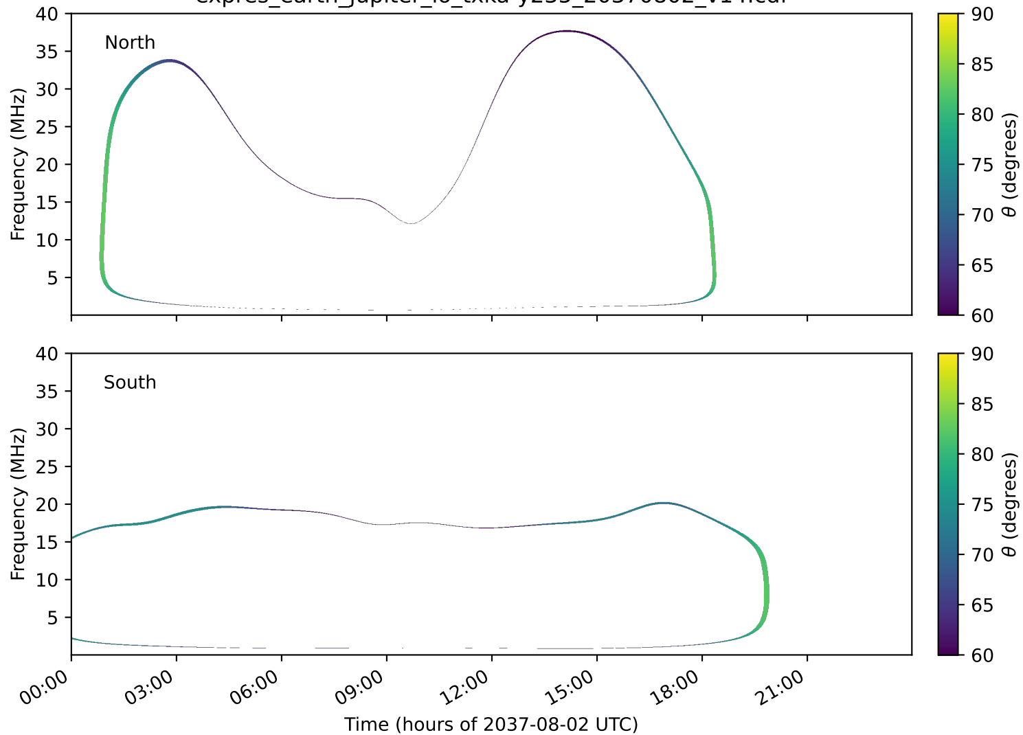
expres_earth_jupiter_io_txka-y235_20370802_v14.cdf
