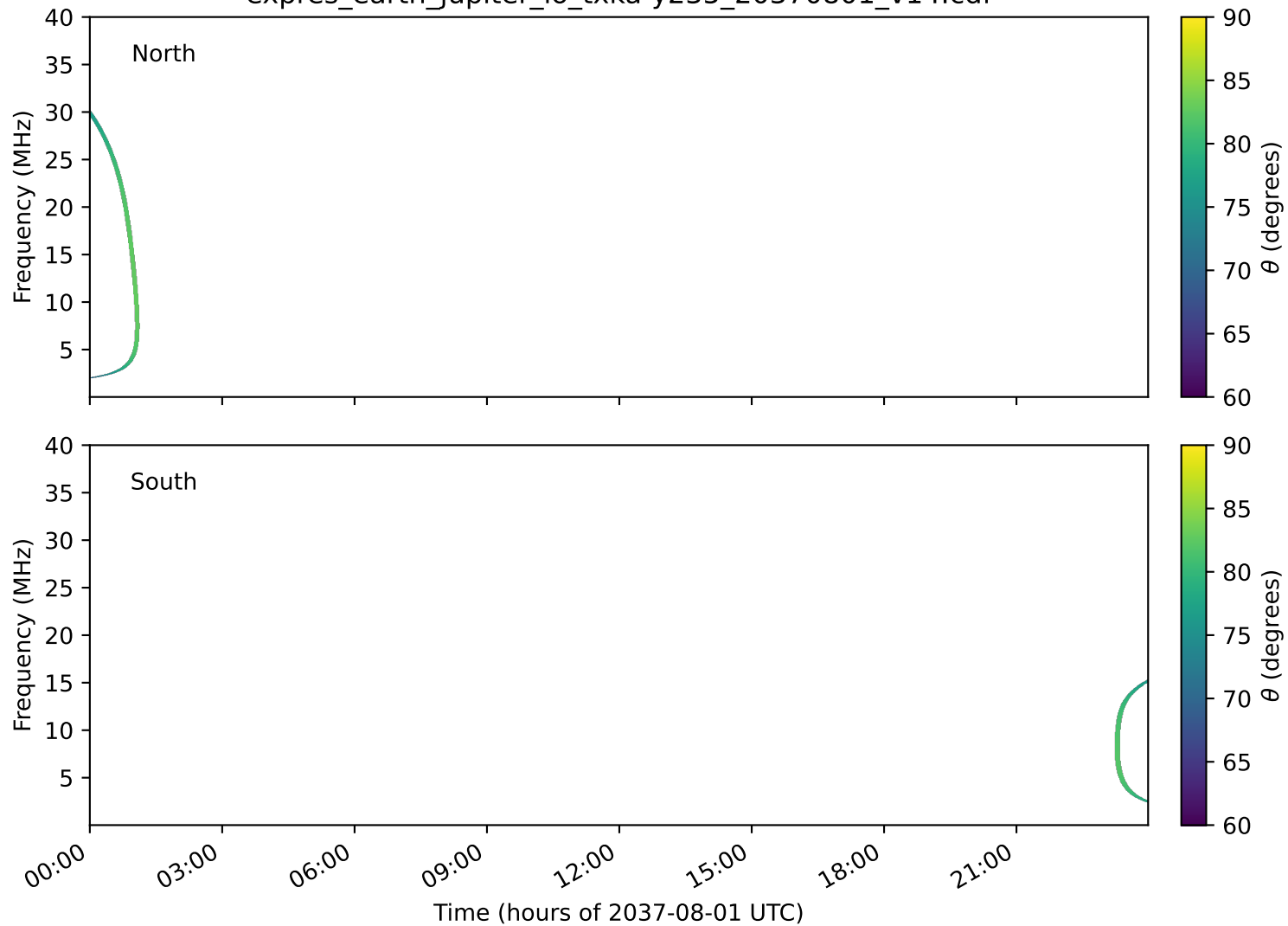
expres_earth_jupiter_io_txka-y235_20370801_v14.cdf
