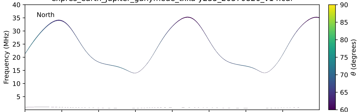
expres_earth_jupiter_ganymede_txka-y235_20370826_v14.cdf
