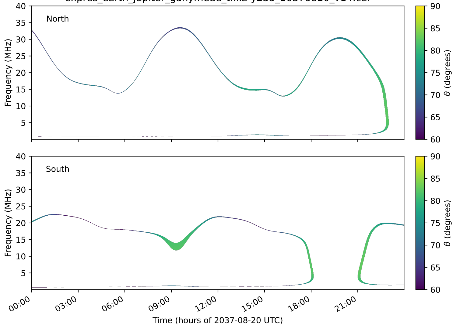
expres_earth_jupiter_ganymede_txka-y235_20370820_v14.cdf
