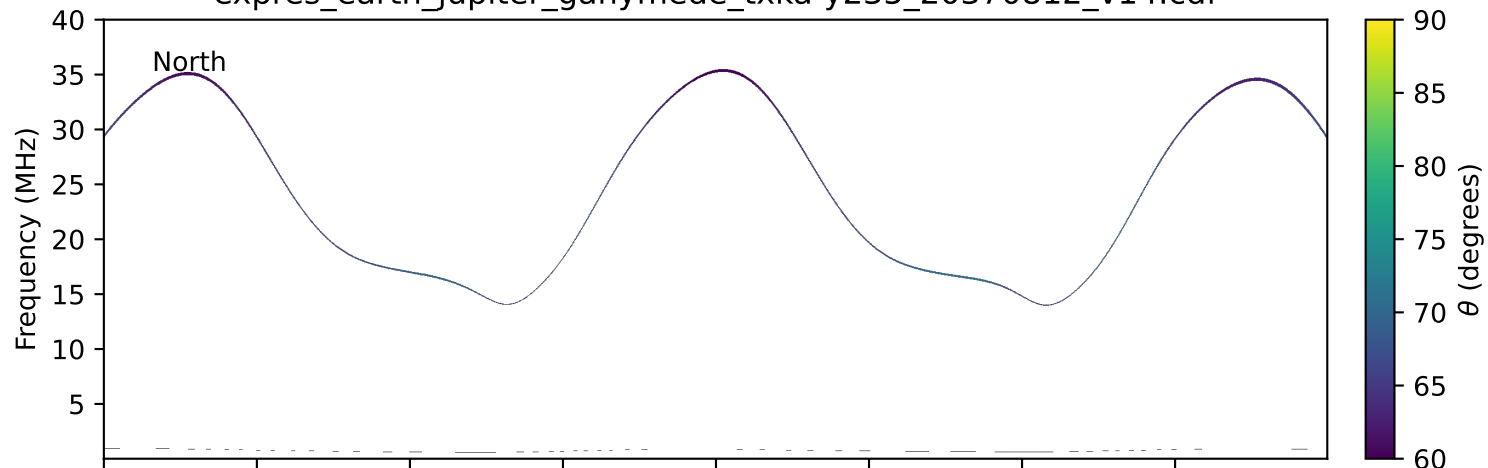
expres_earth_jupiter_ganymede_txka-y235_20370812_v14.cdf
