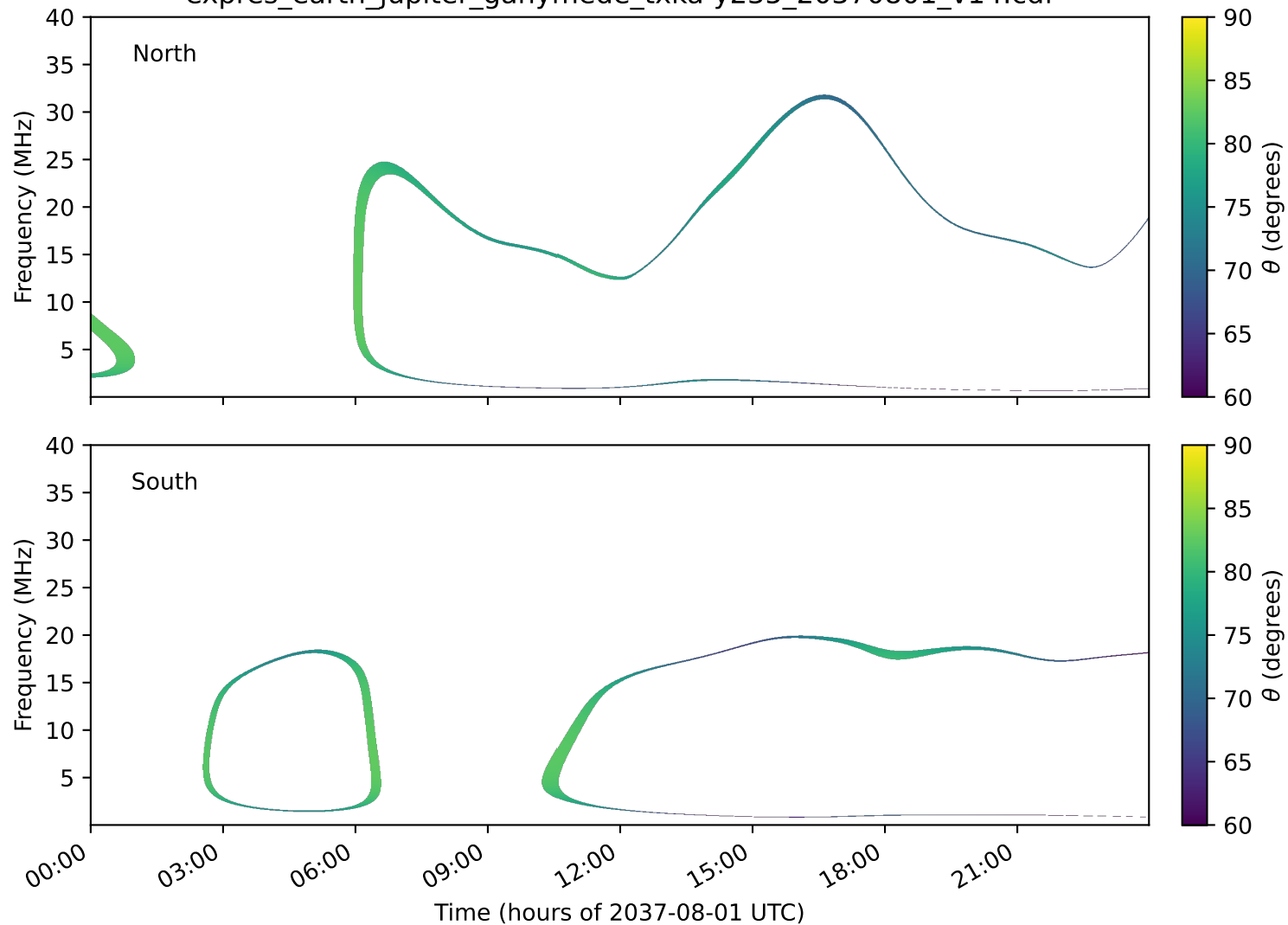
expres_earth_jupiter_ganymede_txka-y235_20370801_v14.cdf
