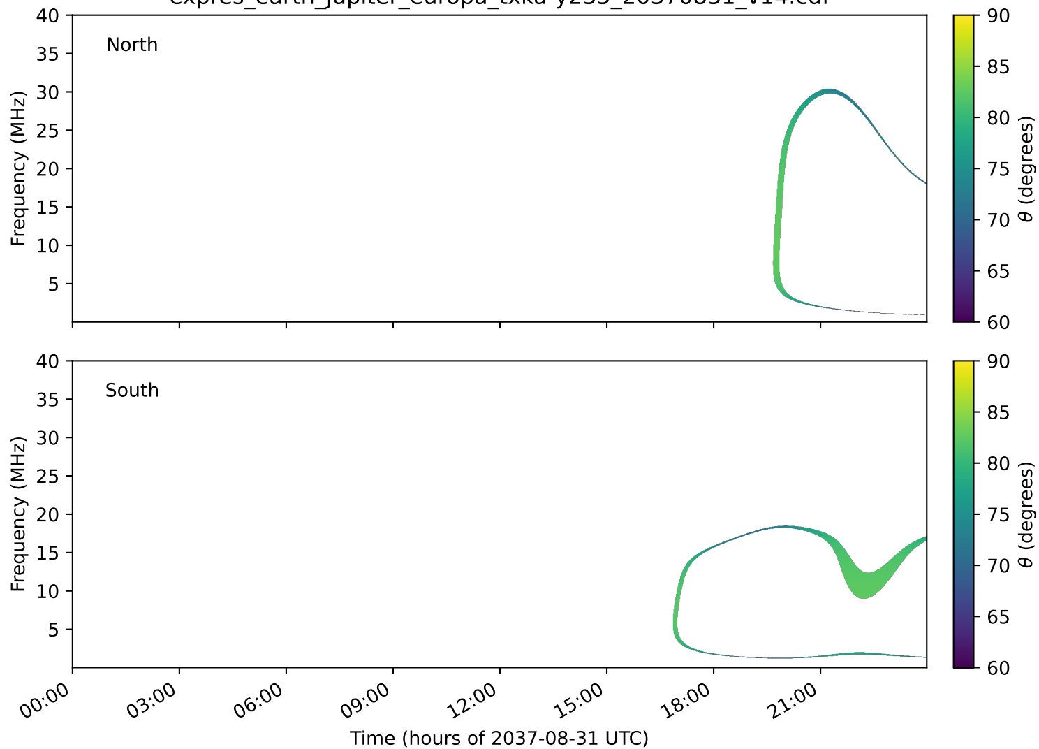
expres_earth_jupiter_europa_txka-y235_20370831_v14.cdf
