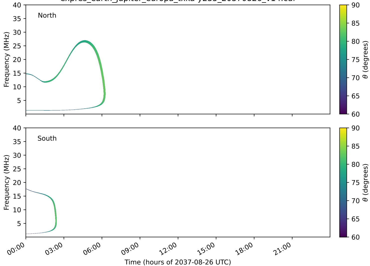
expres_earth_jupiter_europa_txka-y235_20370826_v14.cdf
