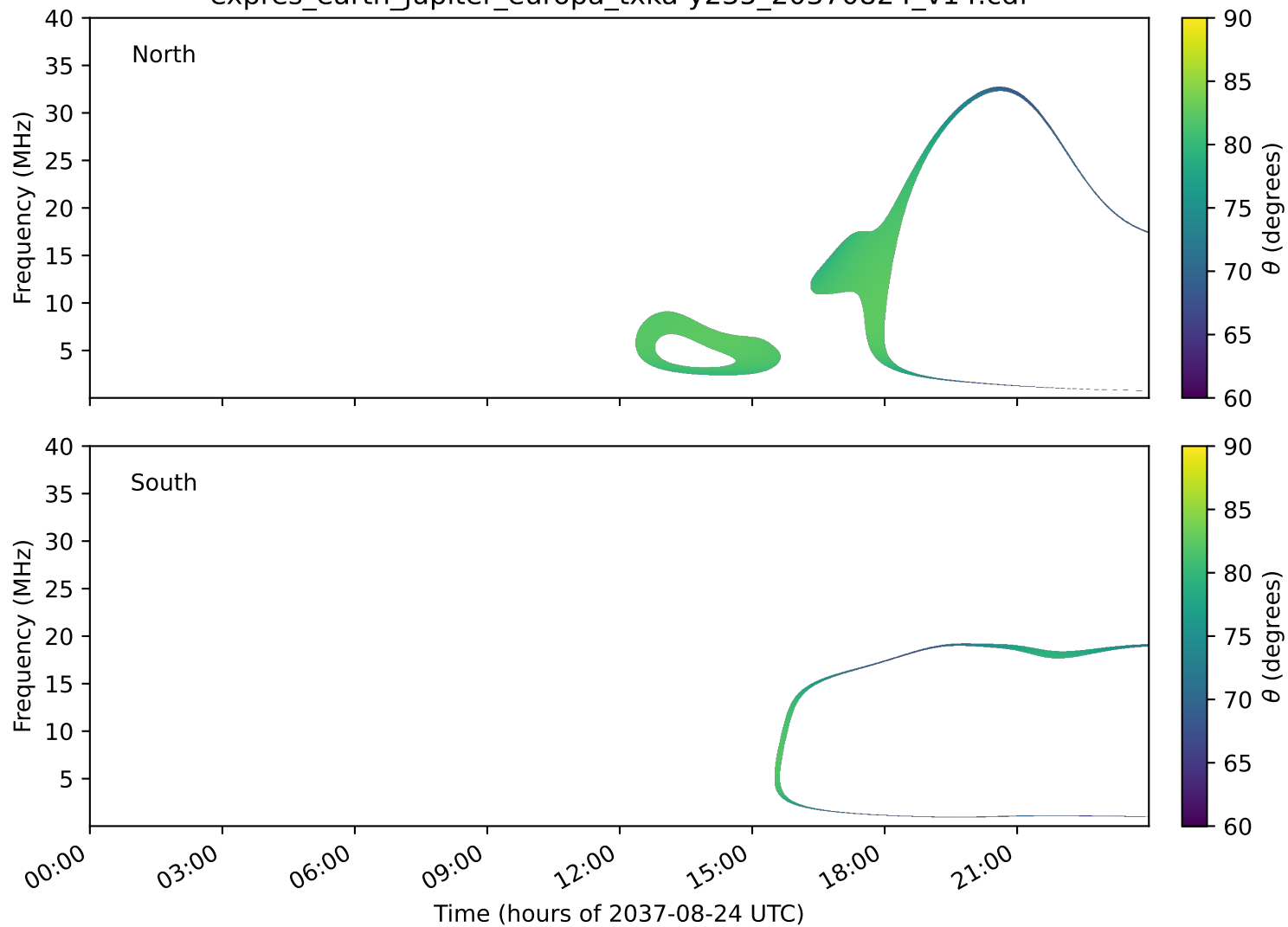
expres_earth_jupiter_europa_txka-y235_20370824_v14.cdf
