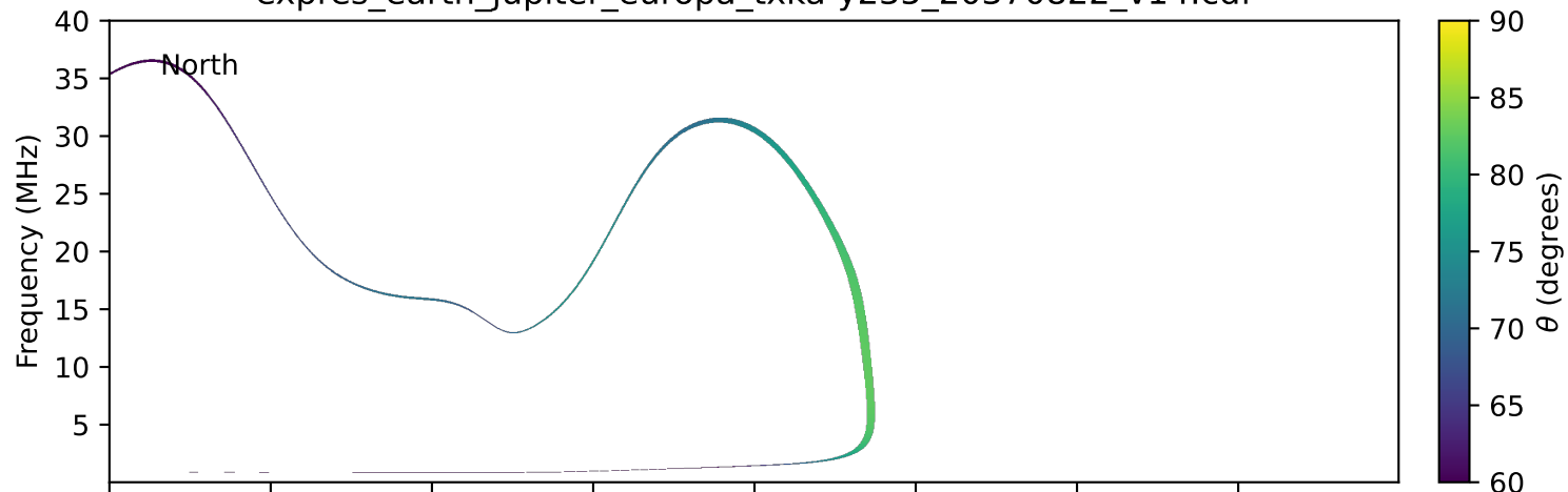
expres_earth_jupiter_europa_txka-y235_20370822_v14.cdf
