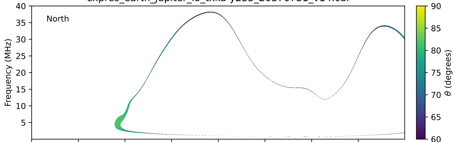
expres_earth_jupiter_io_txka-y235_20370731_v14.cdf
