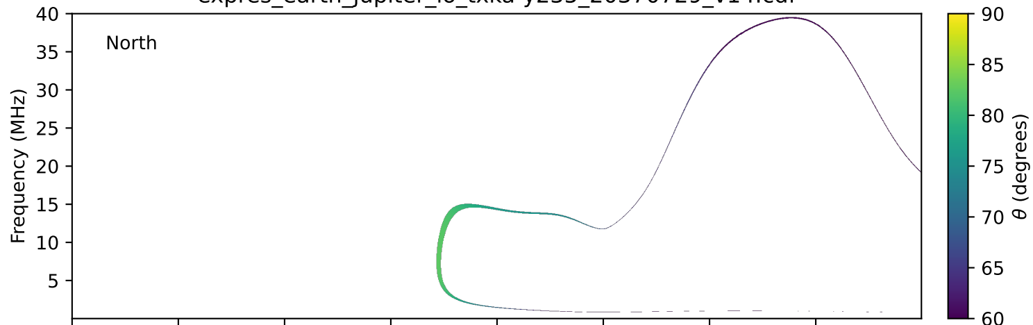
expres_earth_jupiter_io_txka-y235_20370729_v14.cdf
