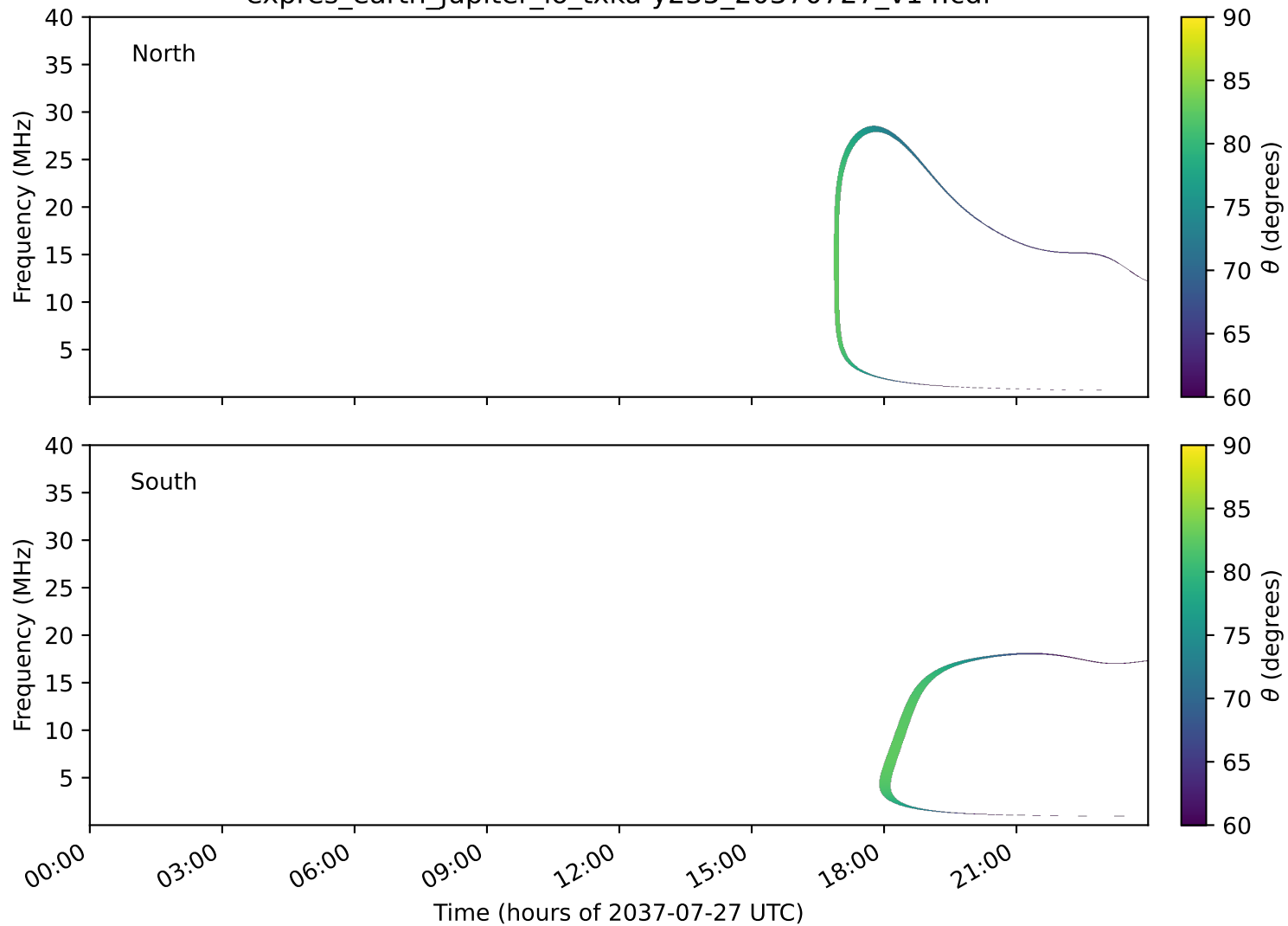
expres_earth_jupiter_io_txka-y235_20370727_v14.cdf
