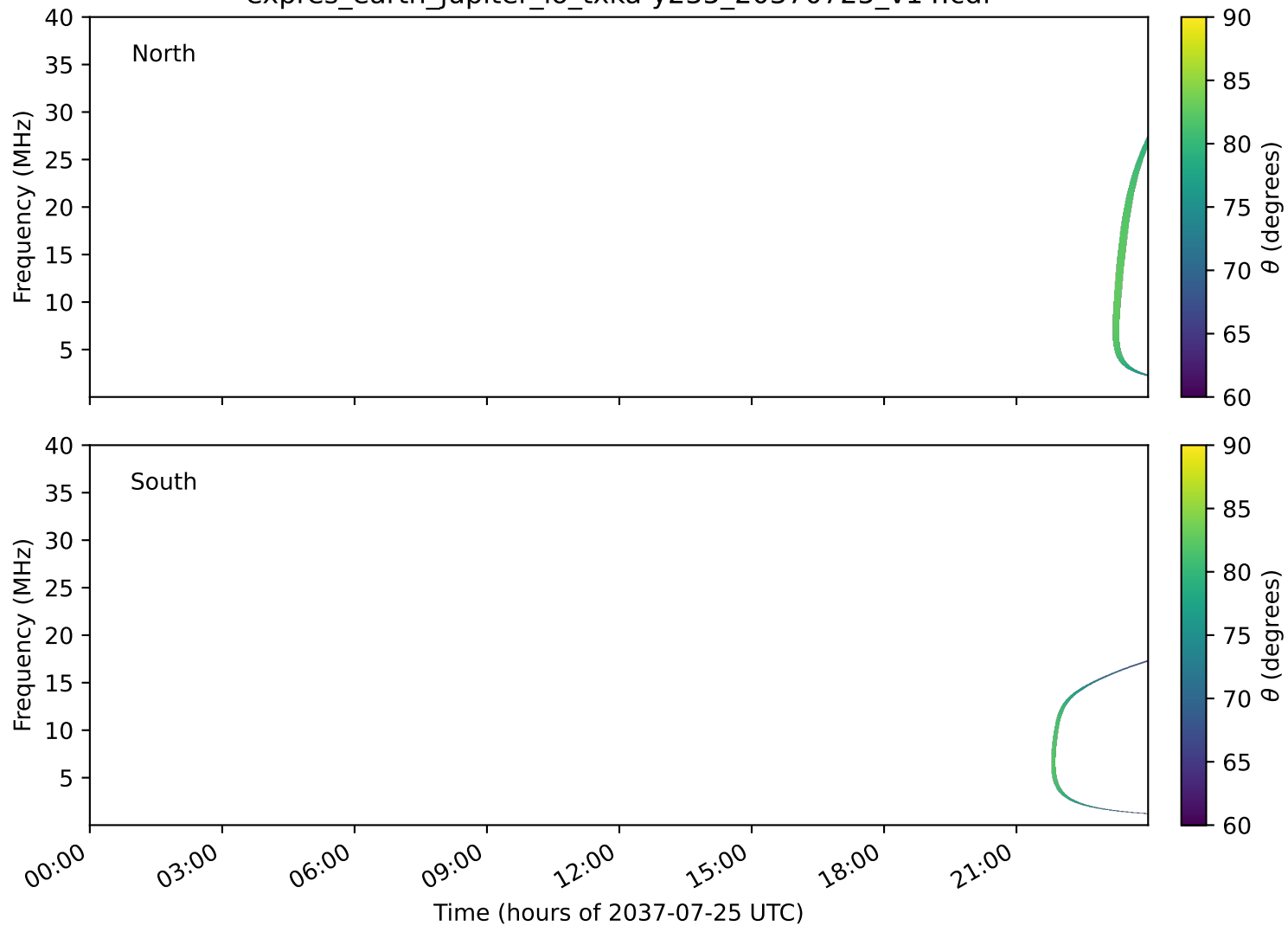
expres_earth_jupiter_io_txka-y235_20370725_v14.cdf
