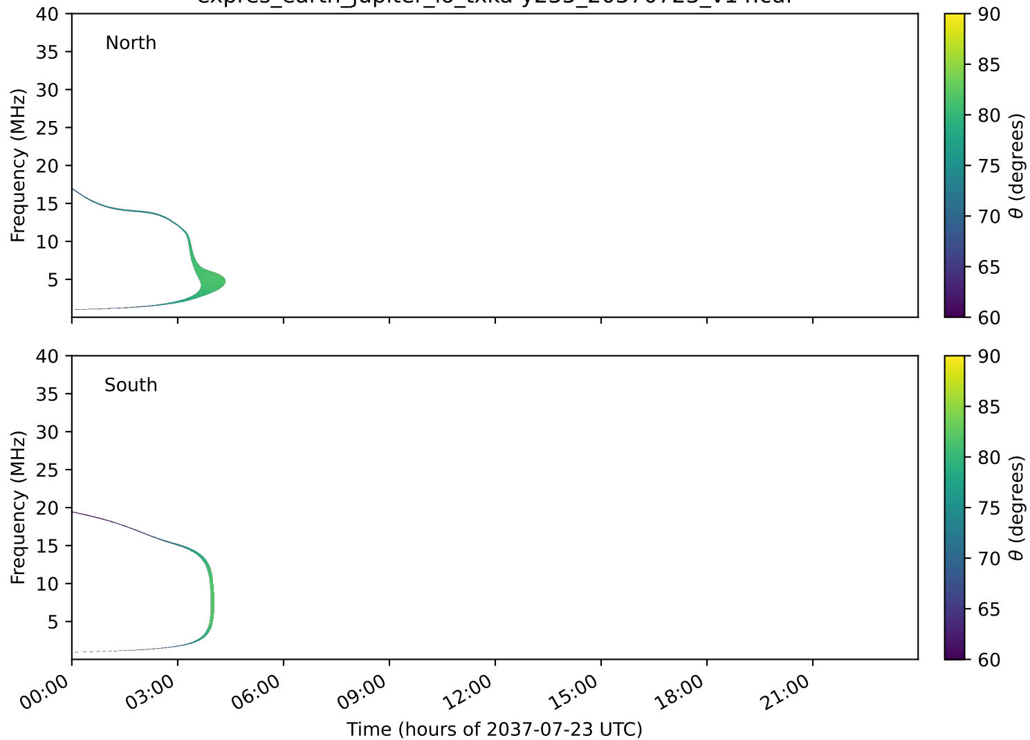
expres_earth_jupiter_io_txka-y235_20370723_v14.cdf
