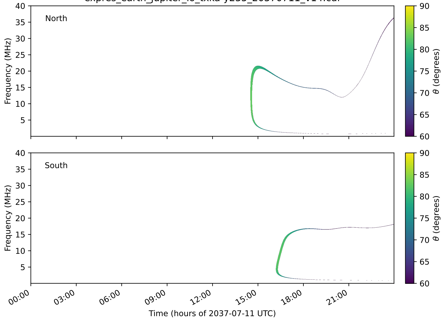
expres_earth_jupiter_io_txka-y235_20370711_v14.cdf
