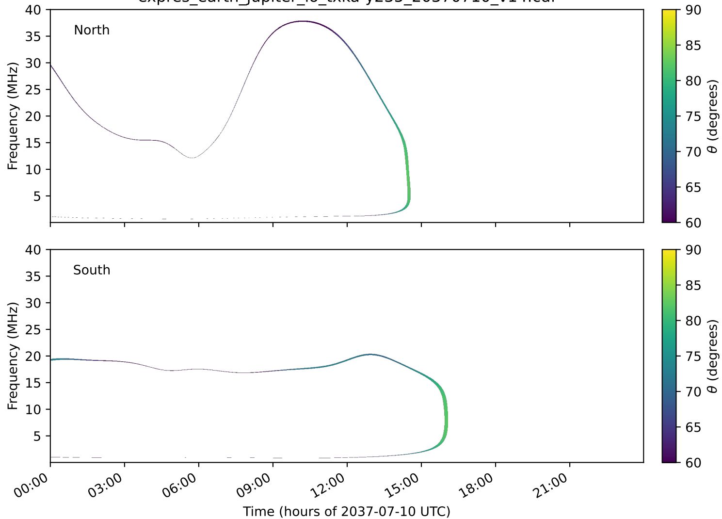
expres_earth_jupiter_io_txka-y235_20370710_v14.cdf
