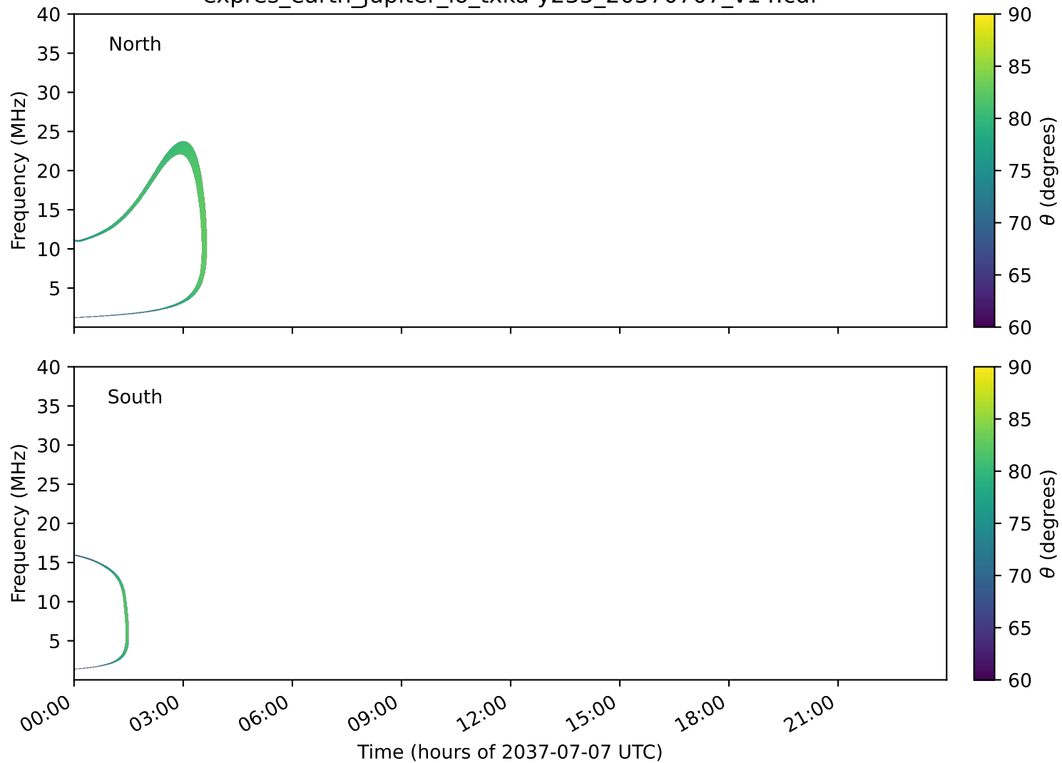
expres_earth_jupiter_io_txka-y235_20370707_v14.cdf
