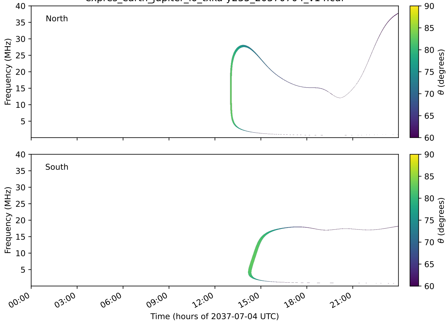
expres_earth_jupiter_io_txka-y235_20370704_v14.cdf
