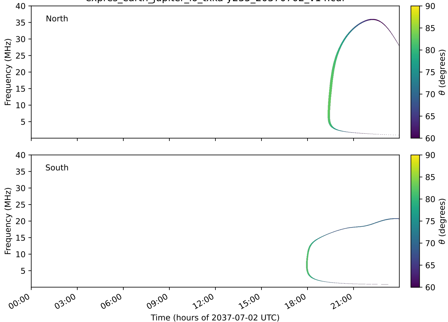
expres_earth_jupiter_io_txka-y235_20370702_v14.cdf
