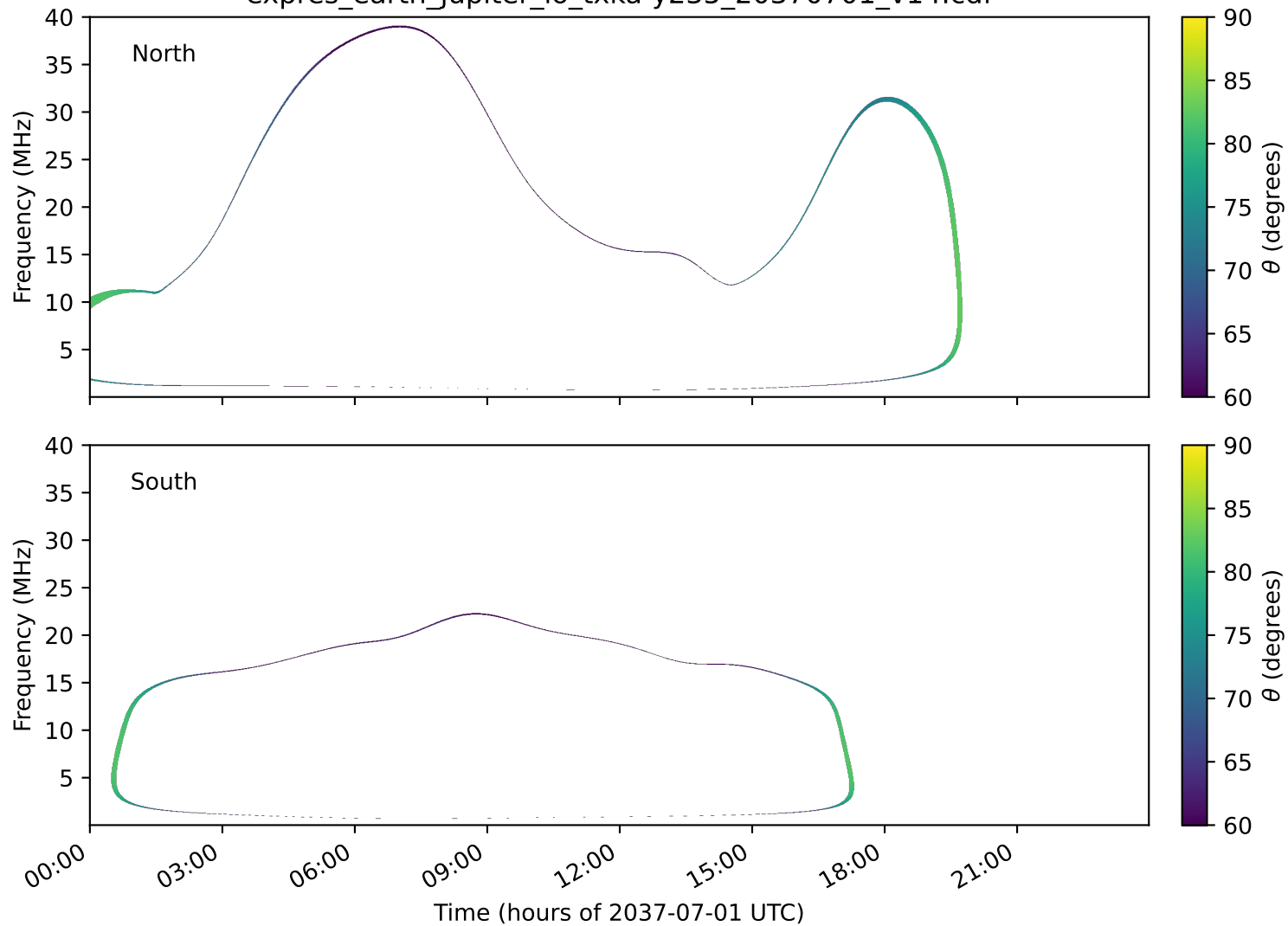
expres_earth_jupiter_io_txka-y235_20370701_v14.cdf
