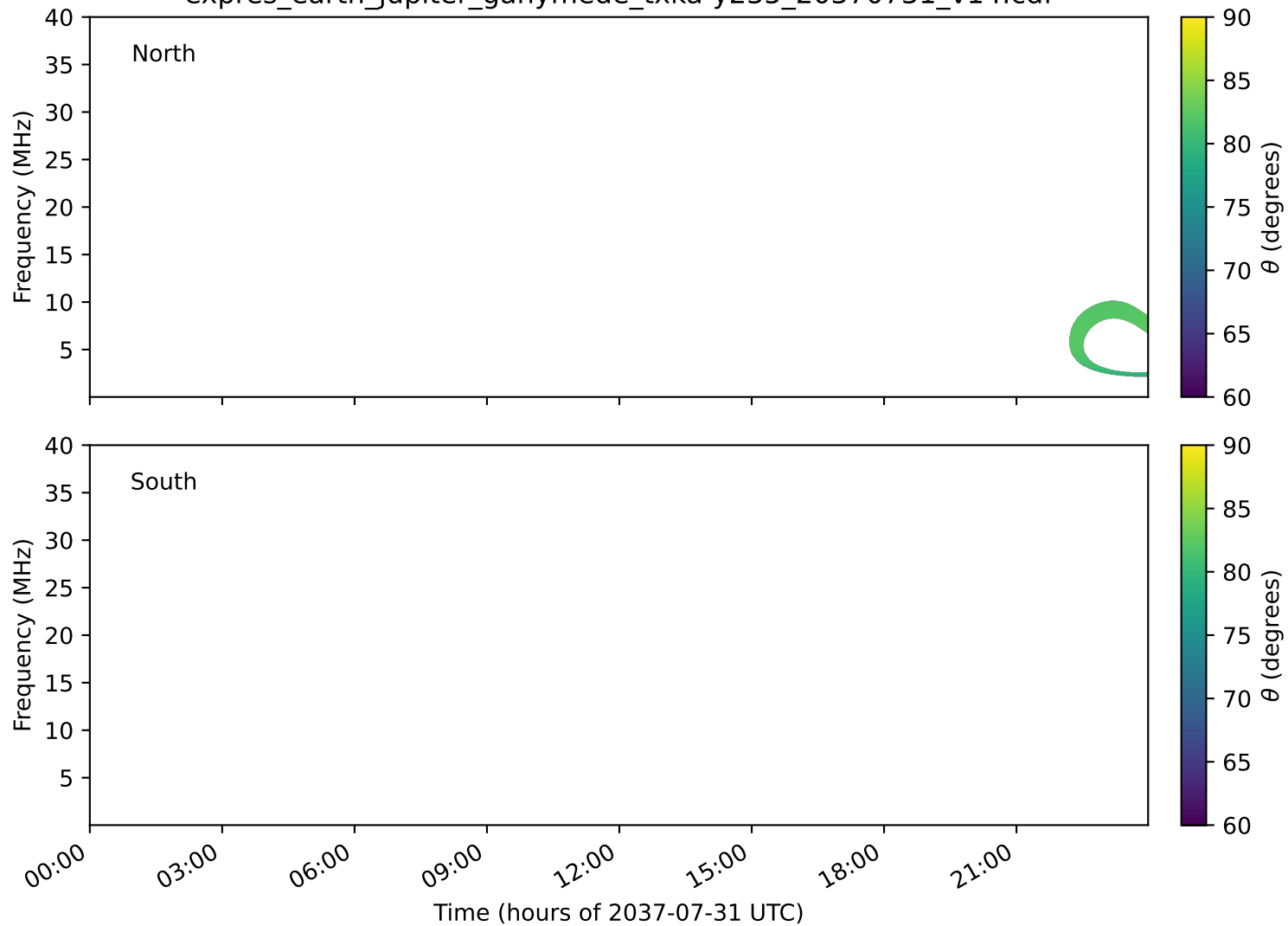
expres_earth_jupiter_ganymede_txka-y235_20370731_v14.cdf
