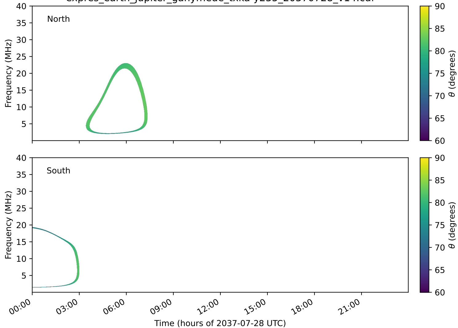
expres_earth_jupiter_ganymede_txka-y235_20370728_v14.cdf
