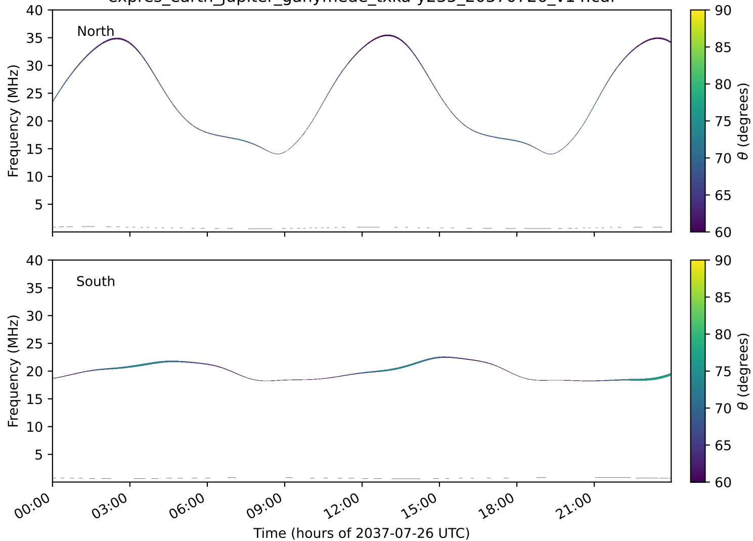
expres_earth_jupiter_ganymede_txka-y235_20370726_v14.cdf
