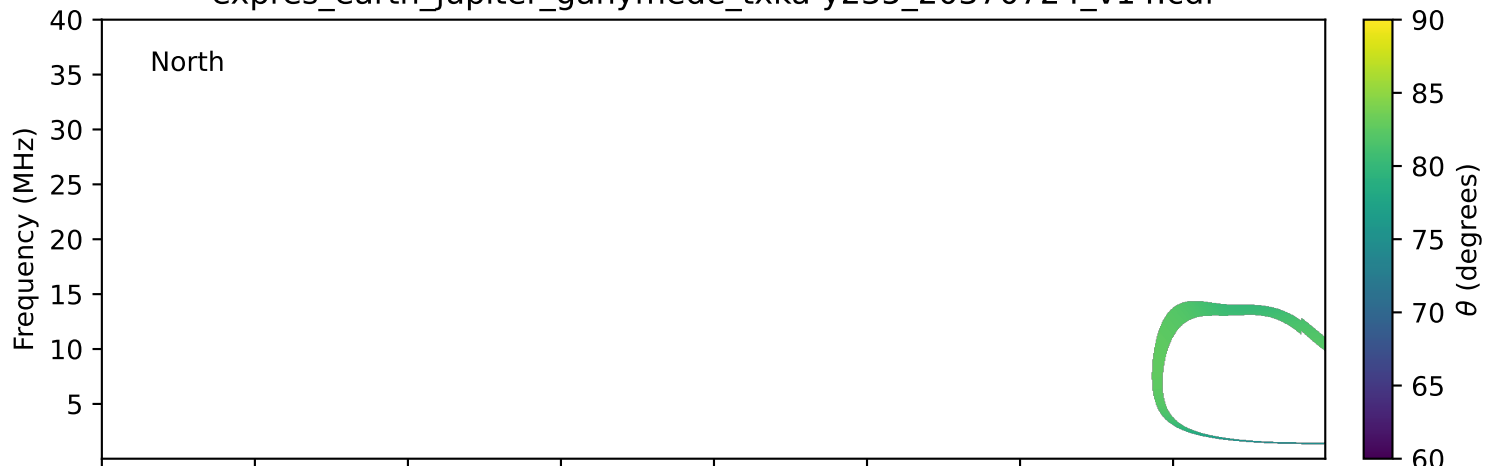
expres_earth_jupiter_ganymede_txka-y235_20370724_v14.cdf
