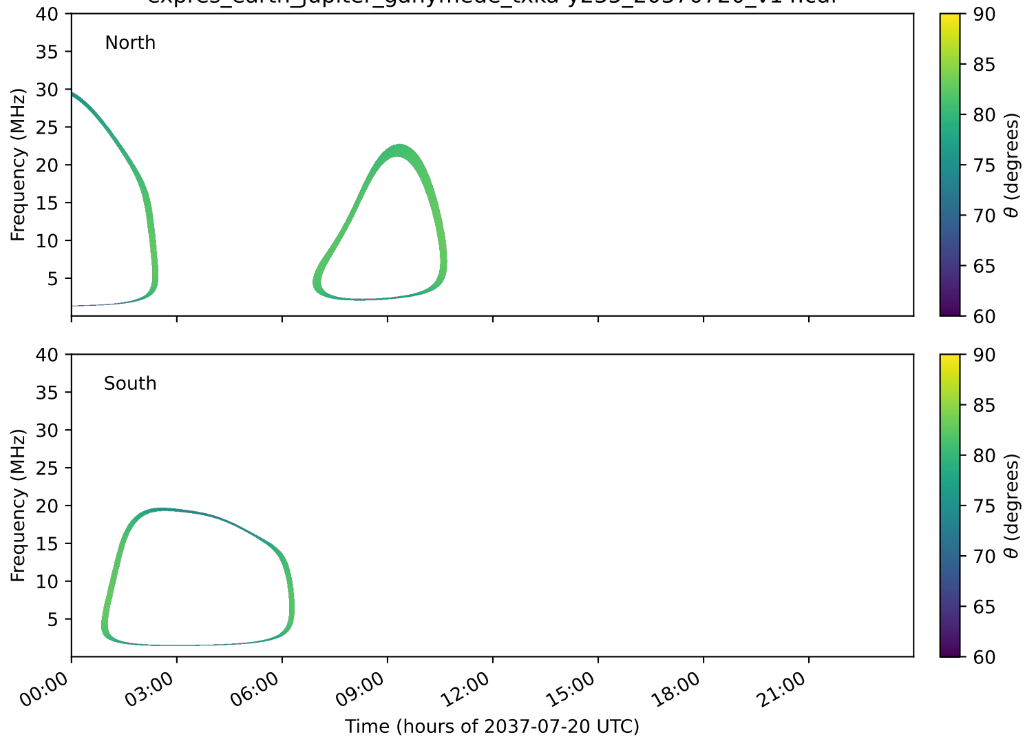
expres_earth_jupiter_ganymede_txka-y235_20370720_v14.cdf
