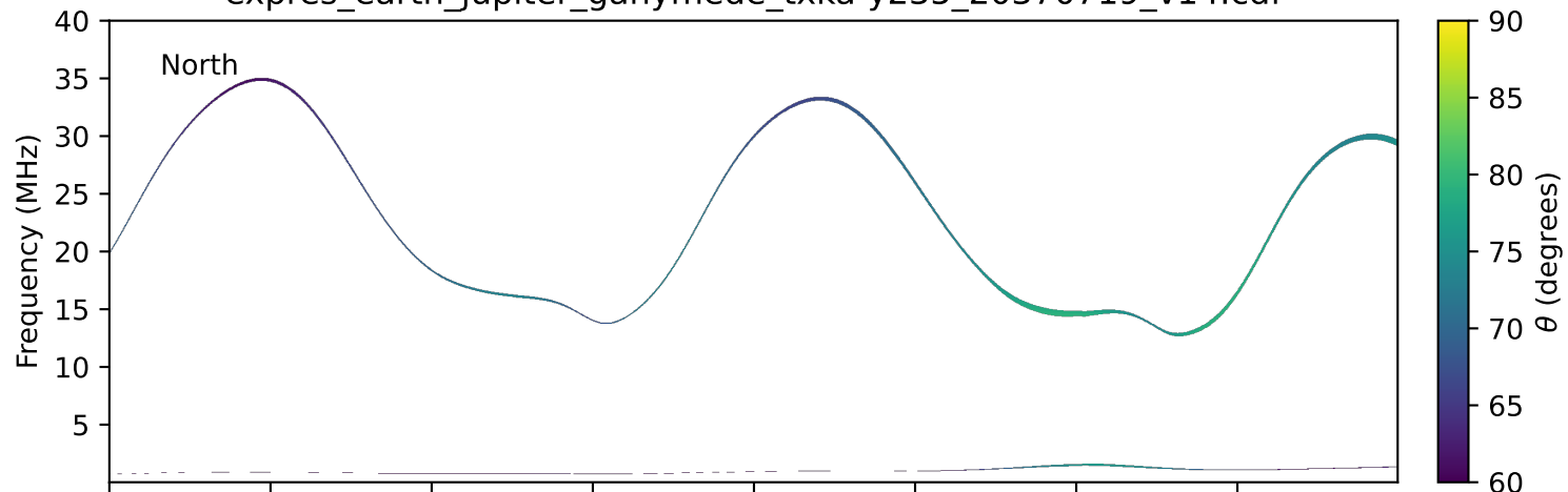
expres_earth_jupiter_ganymede_txka-y235_20370719_v14.cdf
