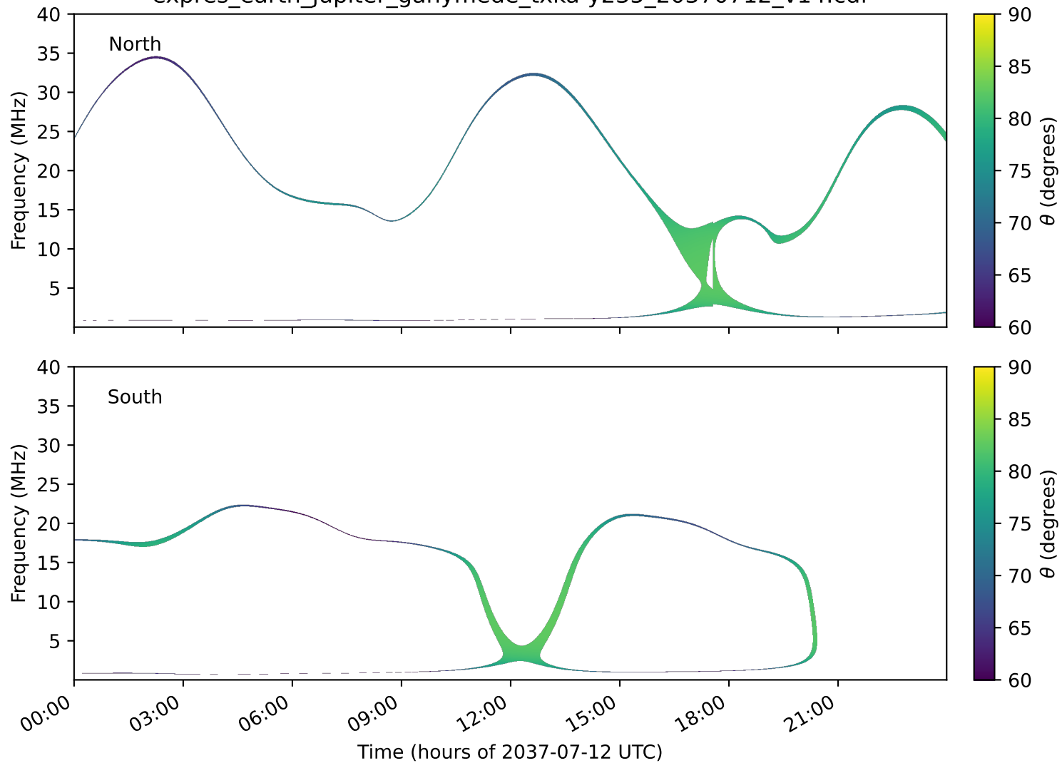
expres_earth_jupiter_ganymede_txka-y235_20370712_v14.cdf
