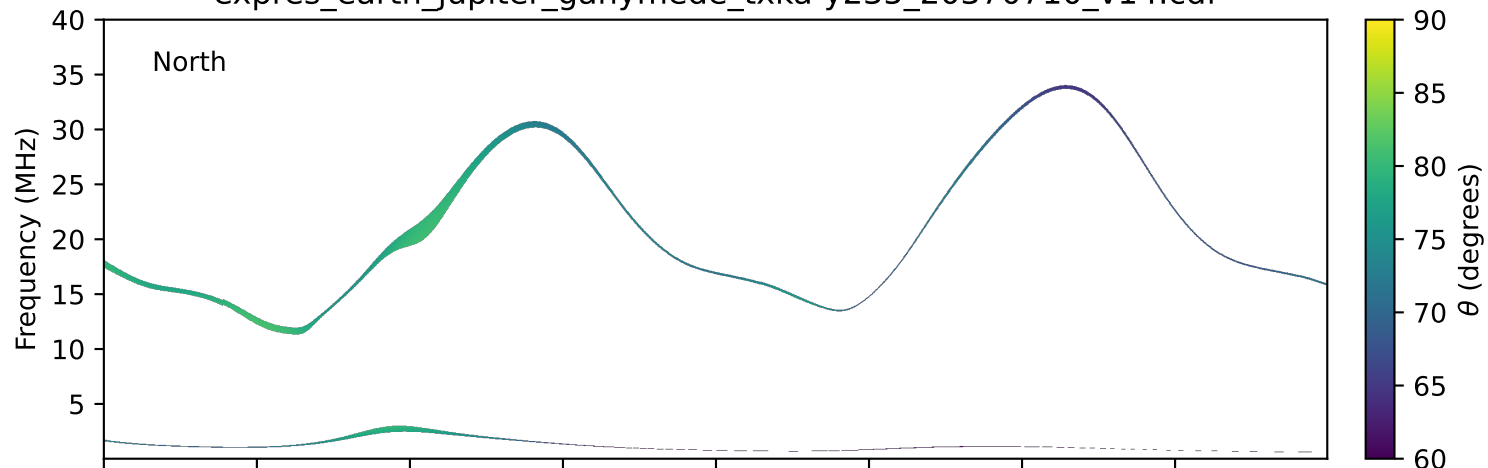
expres_earth_jupiter_ganymede_txka-y235_20370710_v14.cdf
