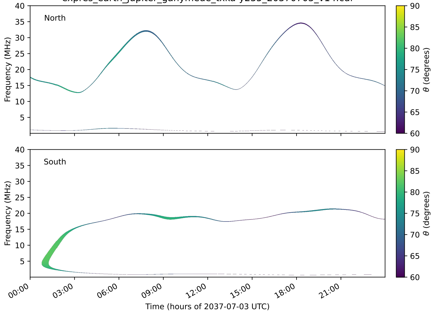
expres_earth_jupiter_ganymede_txka-y235_20370703_v14.cdf
