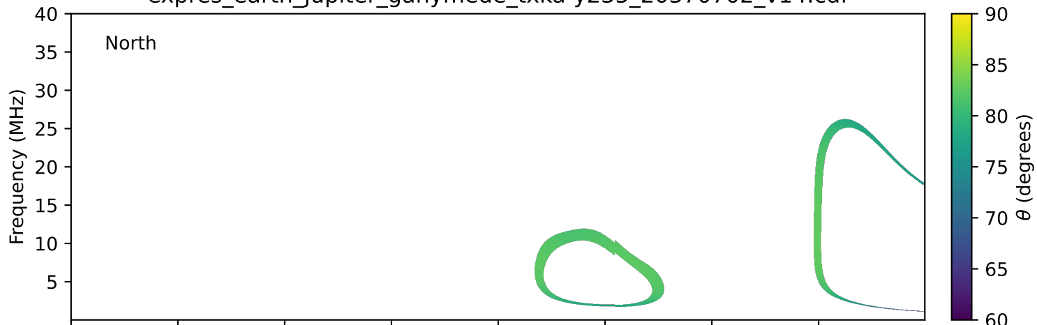
expres_earth_jupiter_ganymede_txka-y235_20370702_v14.cdf
