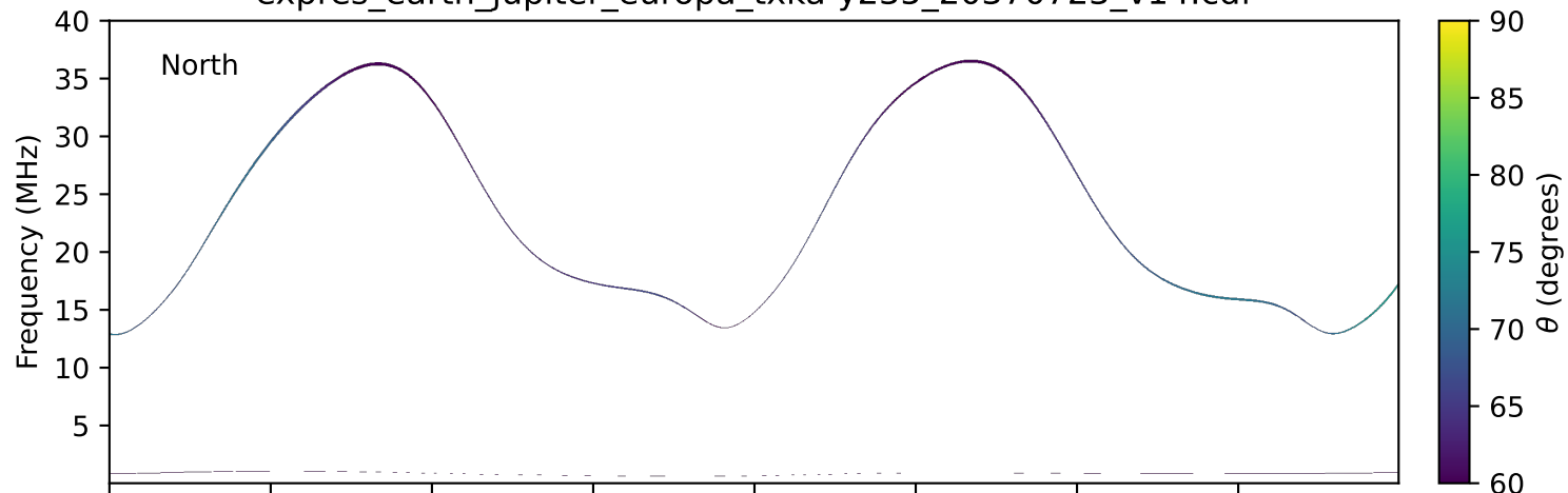
expres_earth_jupiter_europa_txka-y235_20370723_v14.cdf
