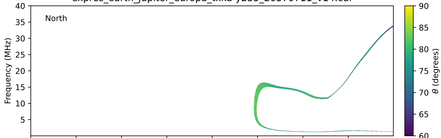
expres_earth_jupiter_europa_txka-y235_20370711_v14.cdf
