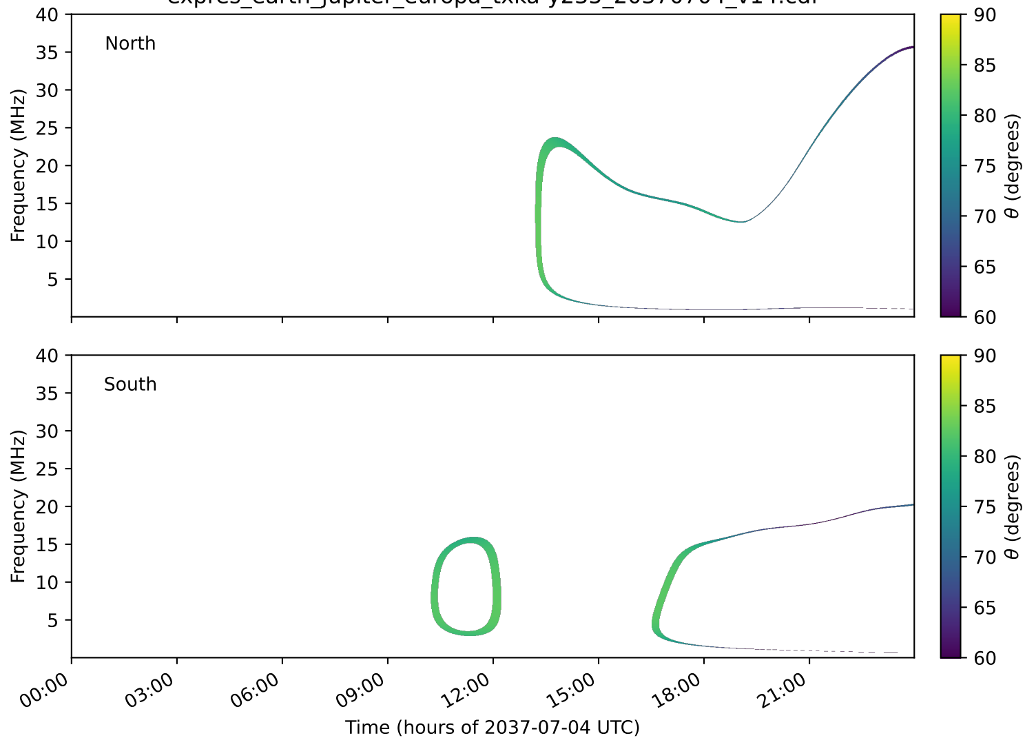
expres_earth_jupiter_europa_txka-y235_20370704_v14.cdf
