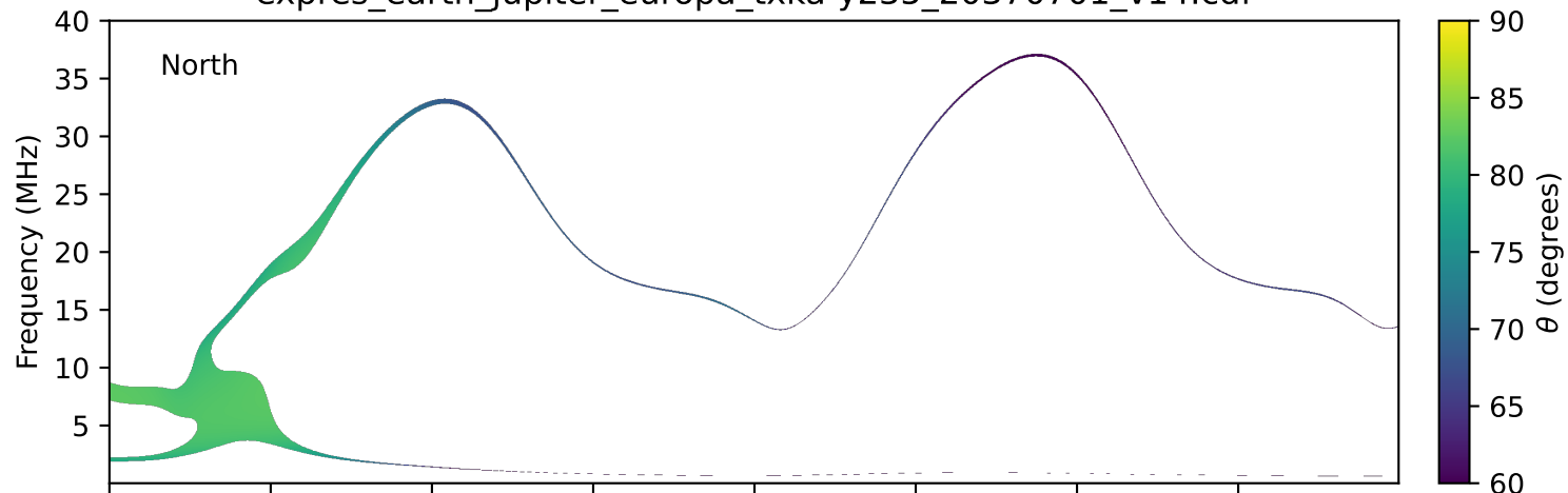
expres_earth_jupiter_europa_txka-y235_20370701_v14.cdf
