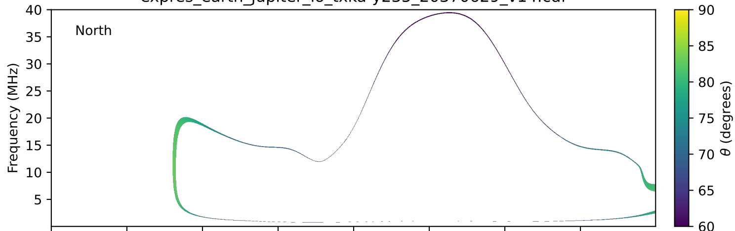
expres_earth_jupiter_io_txka-y235_20370629_v14.cdf
