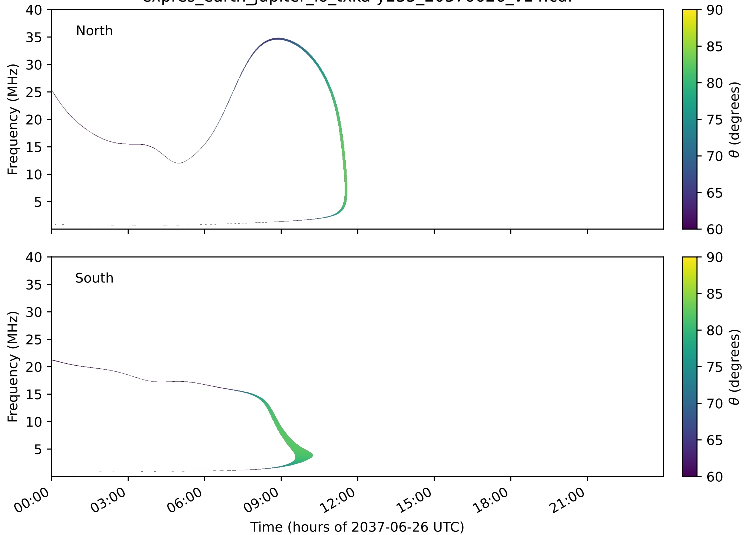
expres_earth_jupiter_io_txka-y235_20370626_v14.cdf
