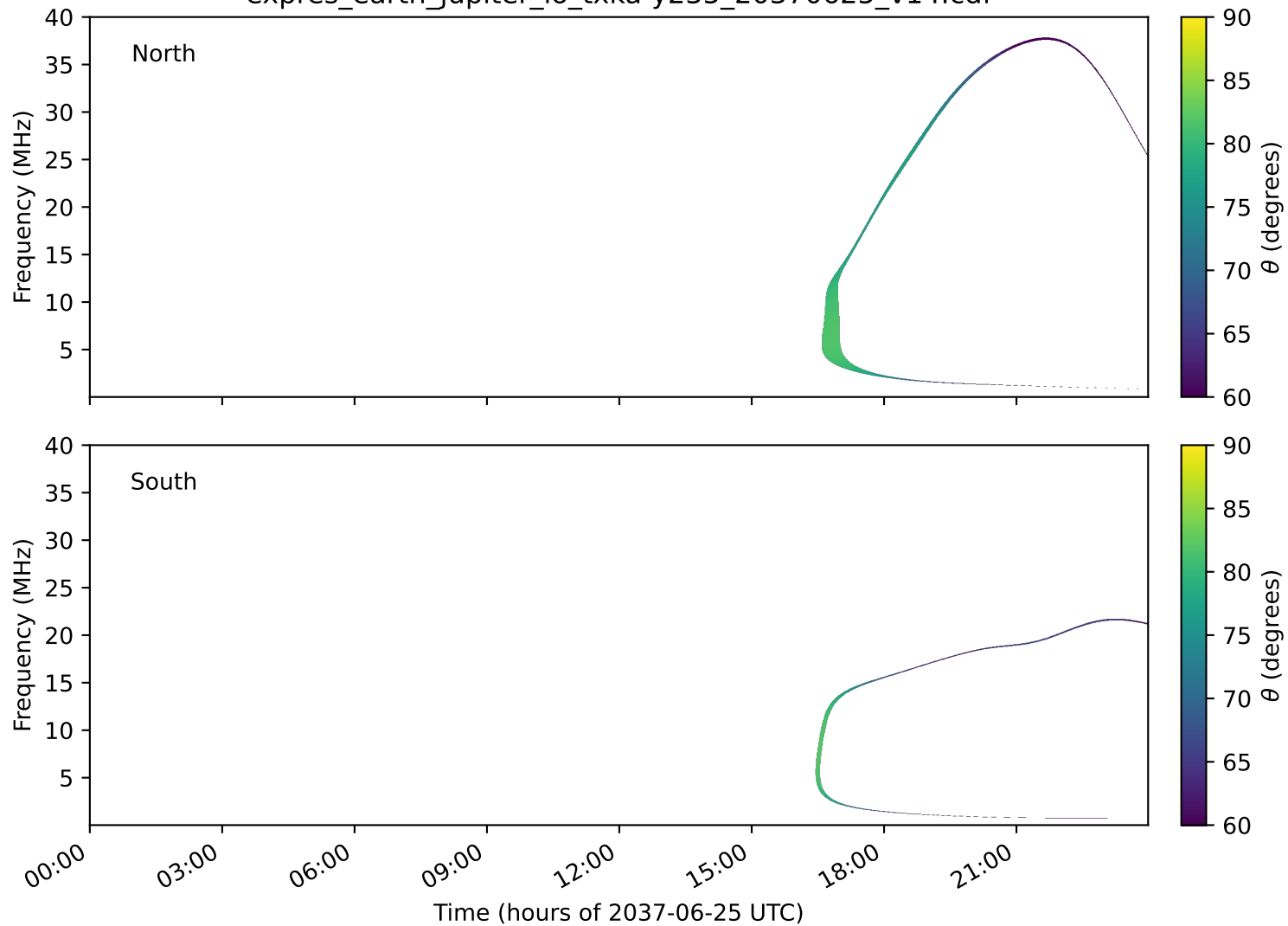
expres_earth_jupiter_io_txka-y235_20370625_v14.cdf
